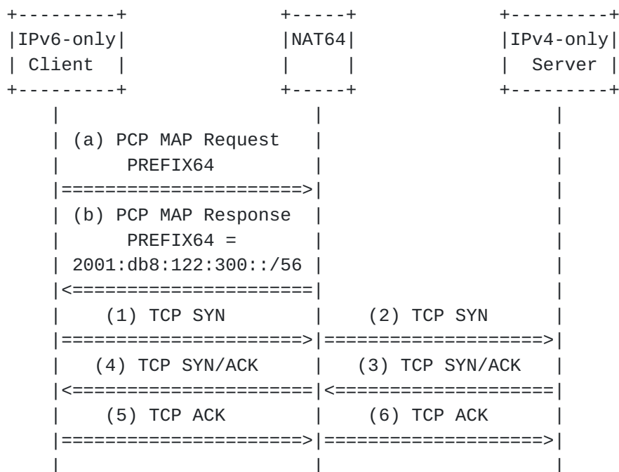
Figure 3: Example of a TCP session initiated from an IPv6-only host
