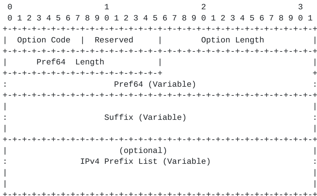
Figure 1: Prefix64 PCP Option
