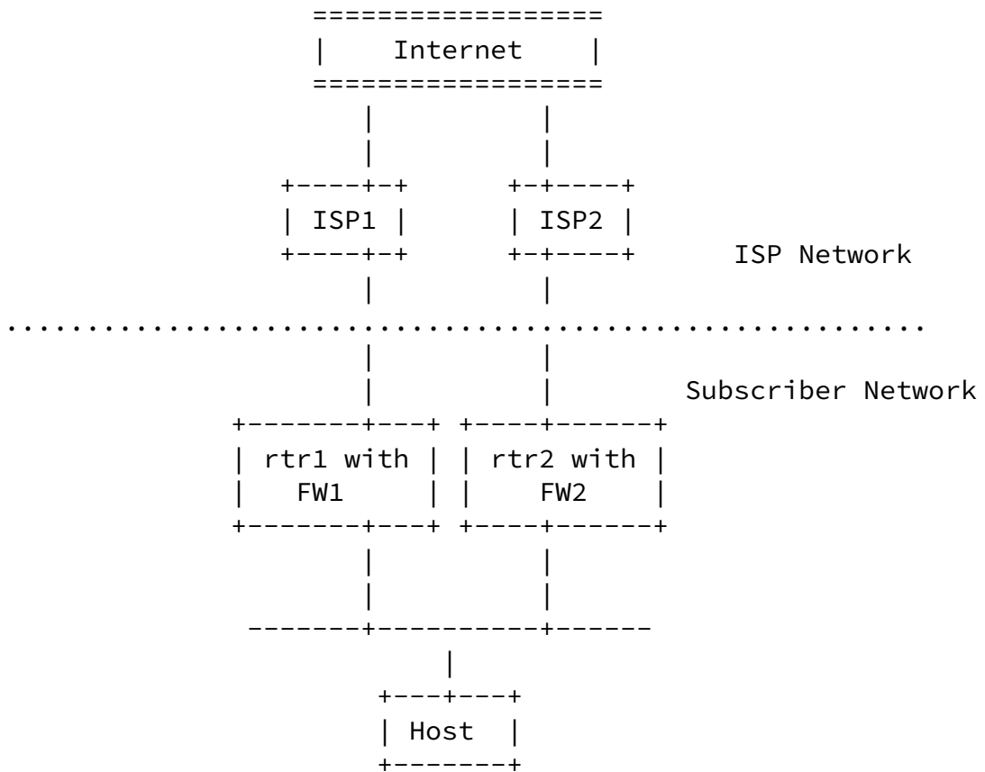
Figure 2: IPv6 Multihoming
