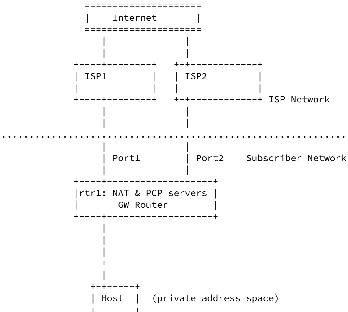
Figure 3: IPv4 Multihoming
