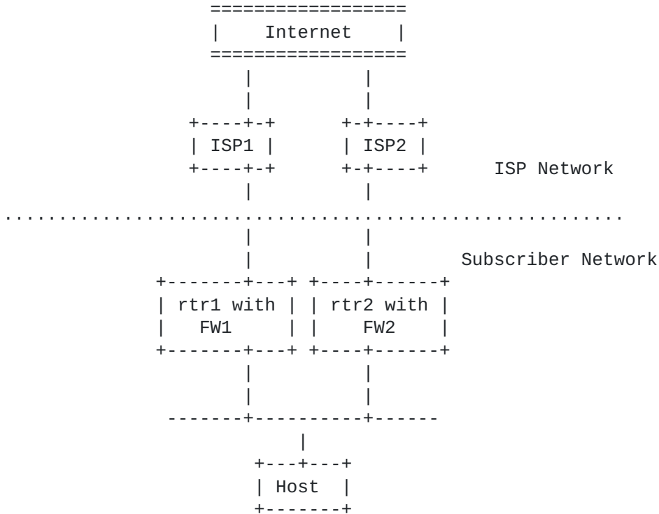
Figure 2: IPv6 Multihoming
