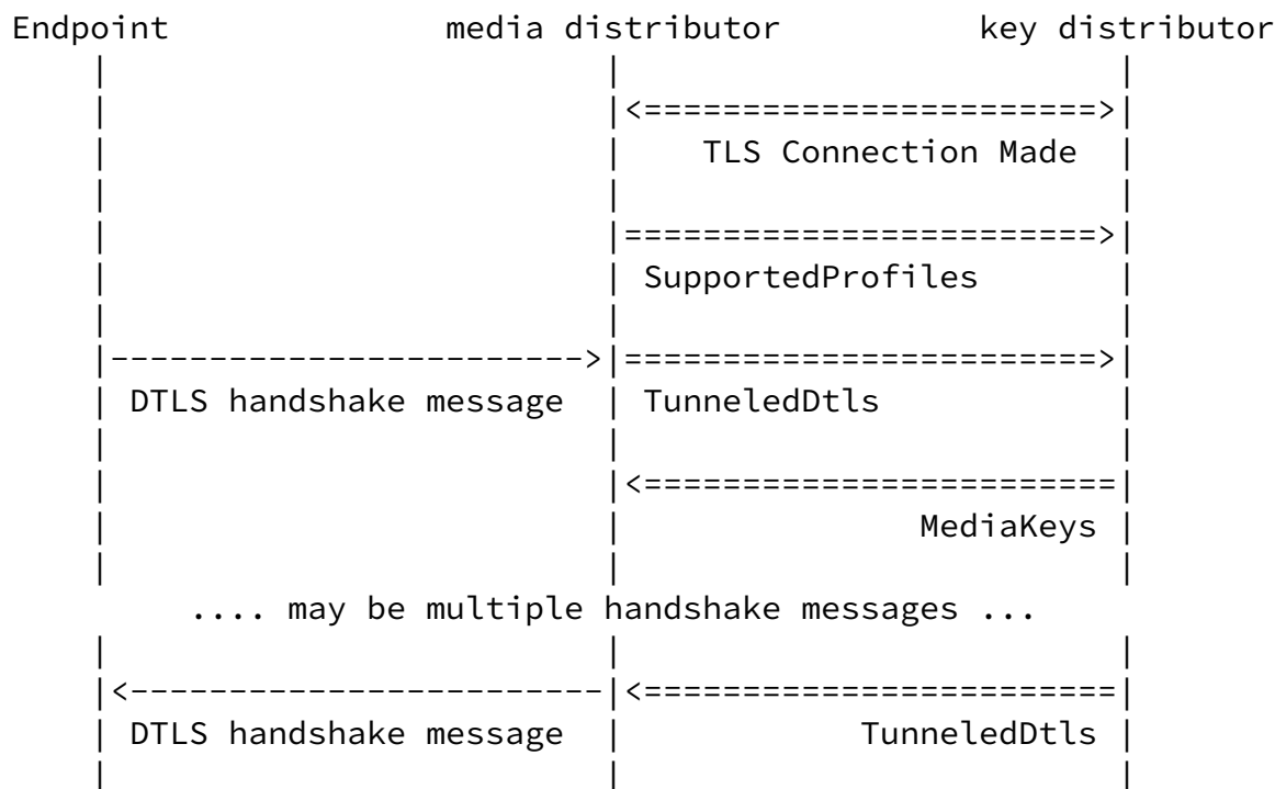
Figure 2: Sample DTLS-SRTP Exchange via the Tunnel
