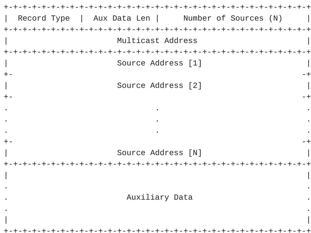
Figure 5: IGMPv3 Report Group Record
