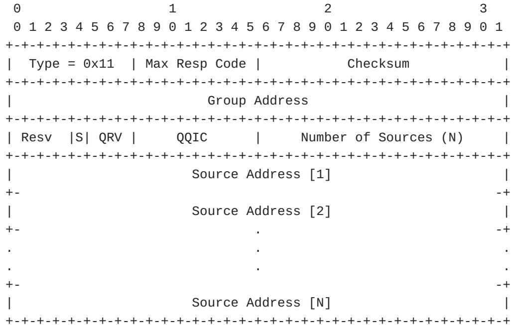
Figure 1: IGMPv3 Query Message
