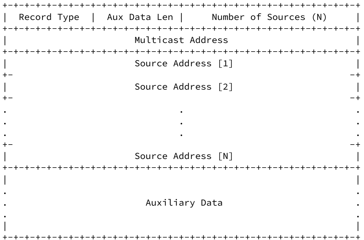
Figure 5: IGMPv3 Report Group Record
