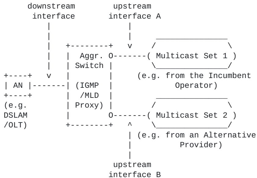
Figure 2: Example of usage of an IGMP/MLD proxy with multiple upstream interfaces in a fixed network scenario
