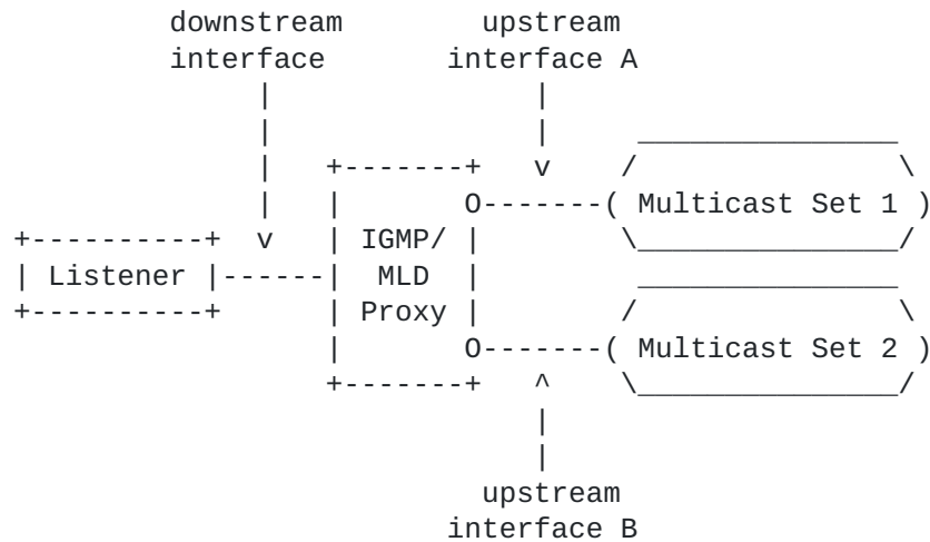
Figure 1: Concept of IGMP/MLD proxy with multiple upstream interfaces
