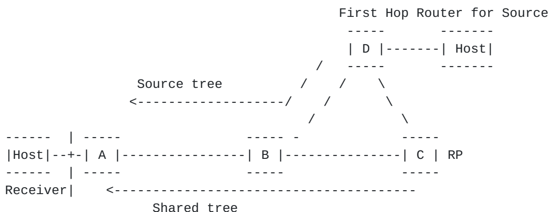
Fig. 3 Example: Switching from shared tree to shortest path tree
