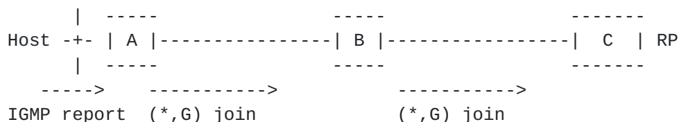
Fig. 1 Example: how a receiver joins, and sets up shared tree
