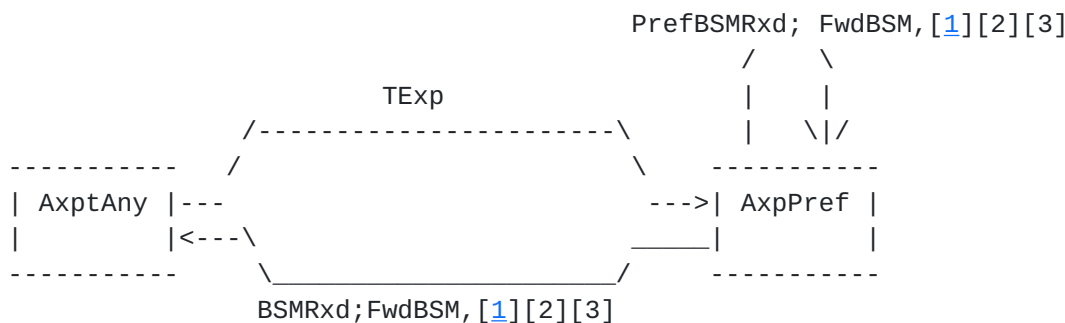
(a) State transition diagram for a candidate BSR
