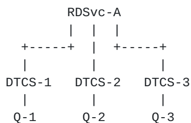
Figure 4. Inputs for a RED Dropper
