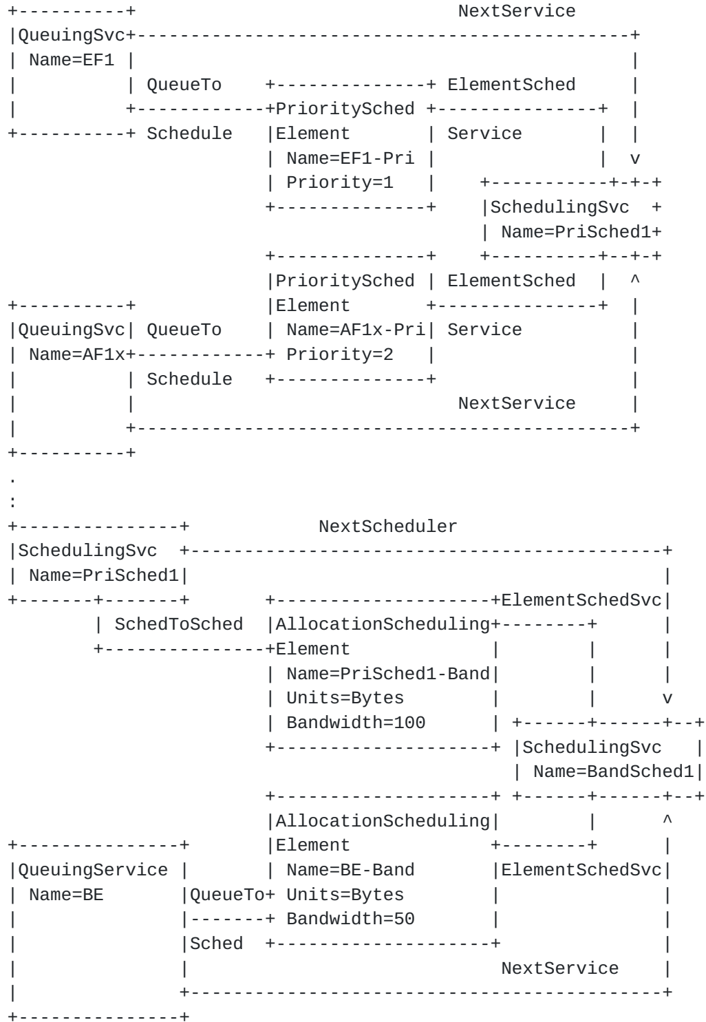
Figure 5. Example 1: Simple Hierarchical Scheduler
