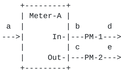
Figure 3: Meter Followed by Two Preamble Markers
