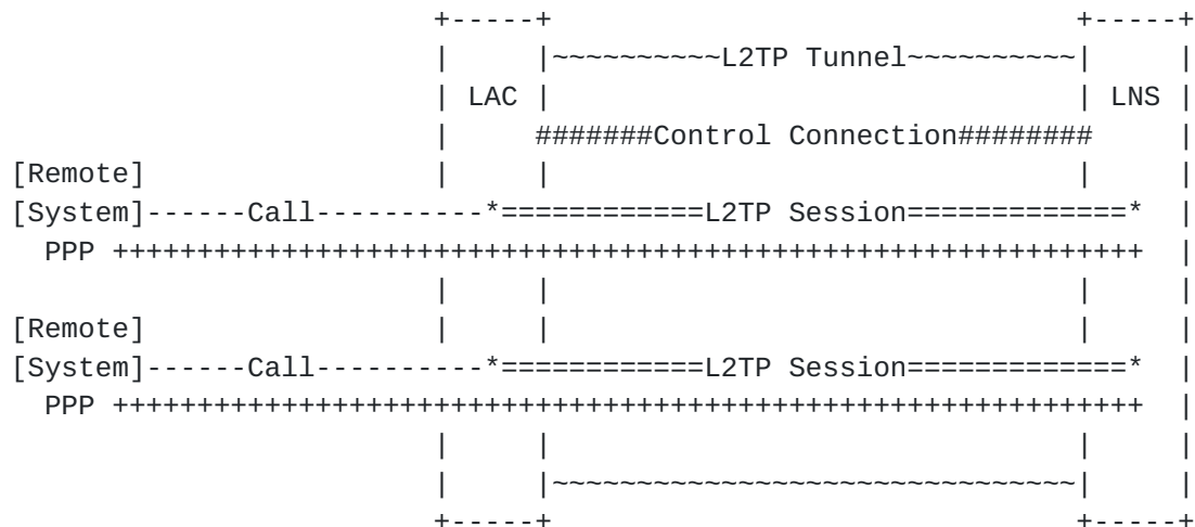
Figure 5.1 Tunneling PPP
