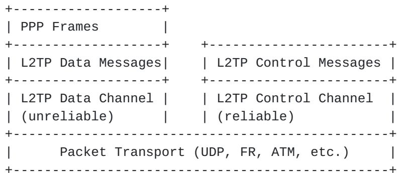
Figure 3.0 L2TP Protocol Structure
