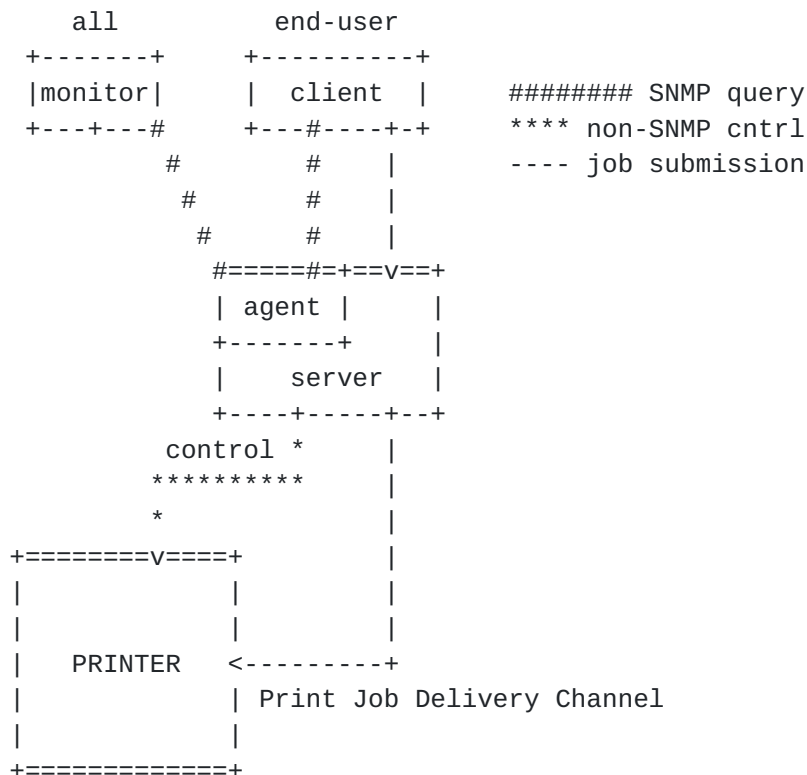
Figure 2-2 - Configuration 2 - client-server-printer - agent in the server
