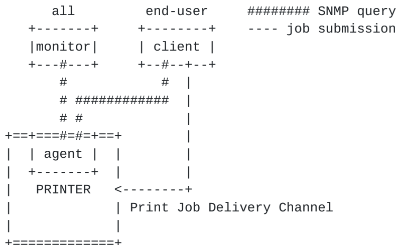
Figure 2-1 - Configuration 1 - client-printer - agent in the printer
