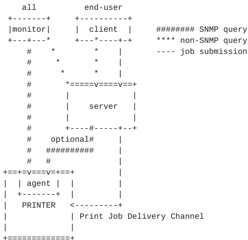
Figure 2-3 - Configuration 3 - client-server-printer - client monitors printer agent and server
