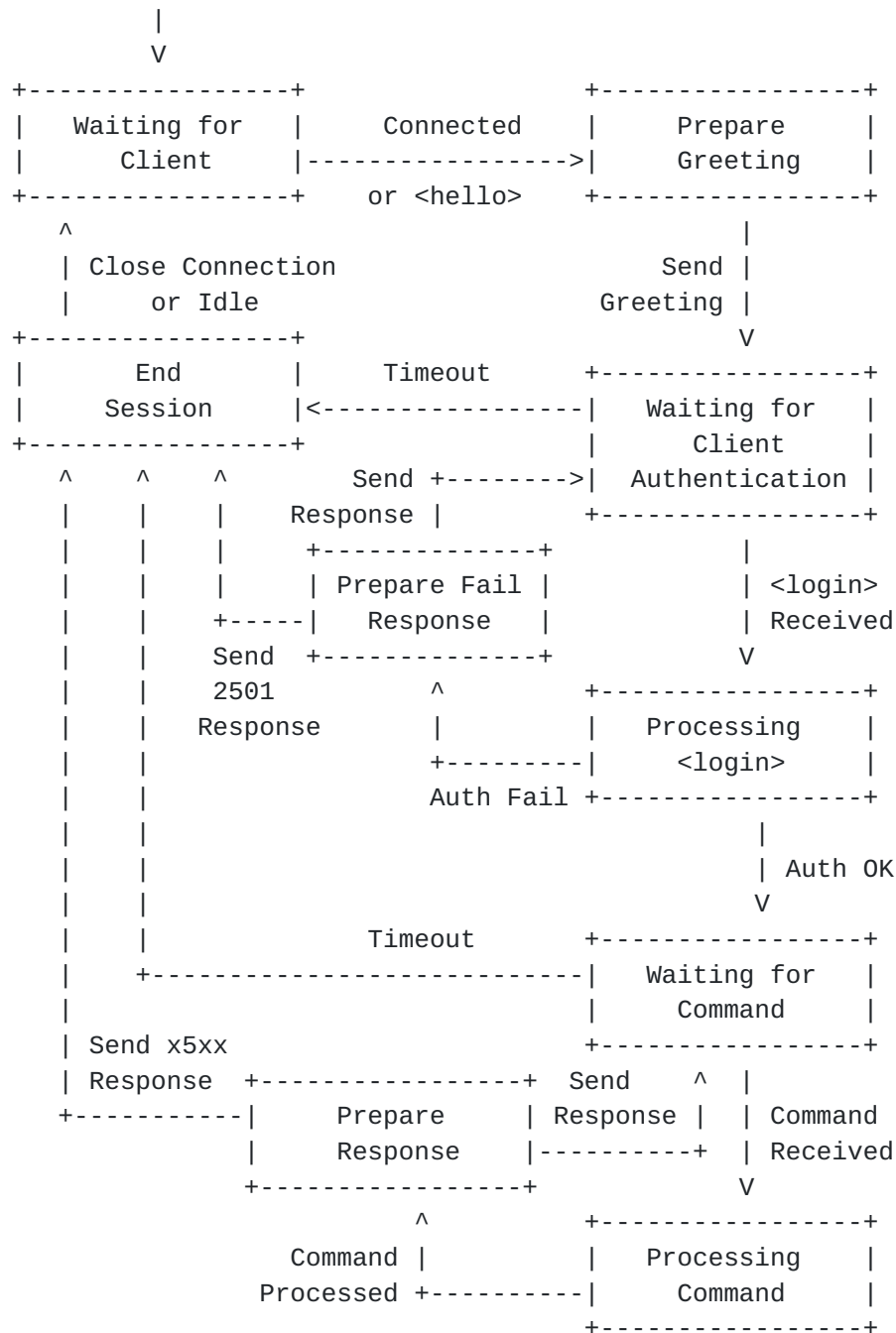
Figure 1: EPP Server State Machine
