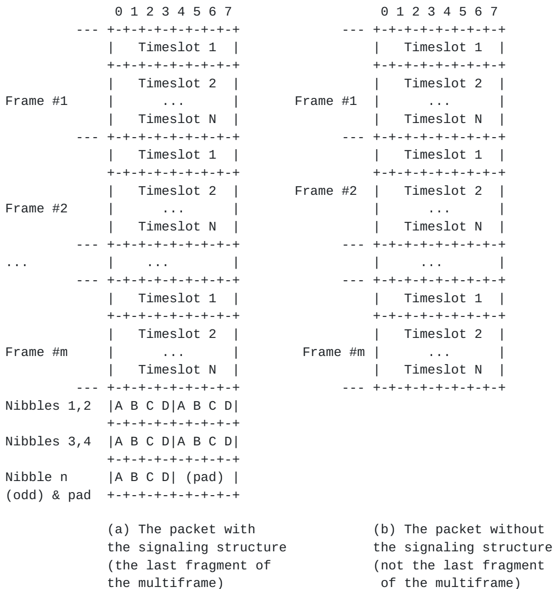
Figure 5. The CESoPSN Packet Payload Format for Trunk-Specific NxDS0 with CAS
