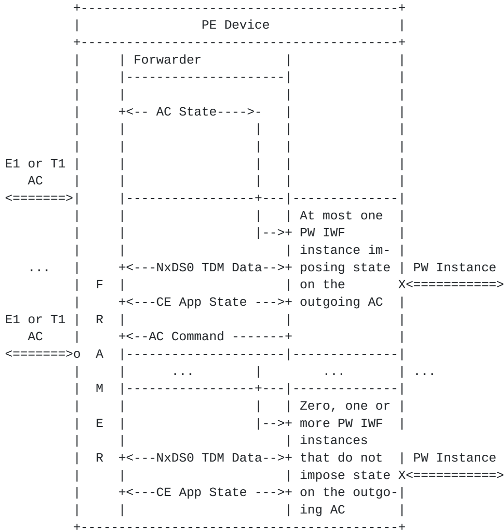
Figure B.1. Reference PE Architecture for NxDS0 Services
