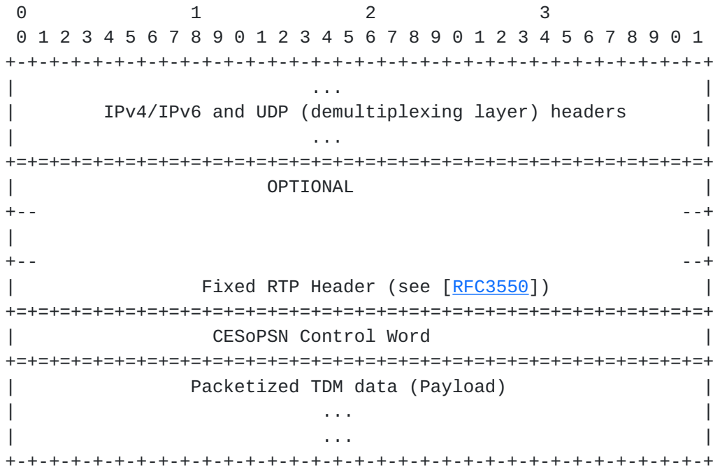
Figure 1a. CESoPSN Packet Format for an IPv4/IPv6 PSN with UDP demultiplexing
