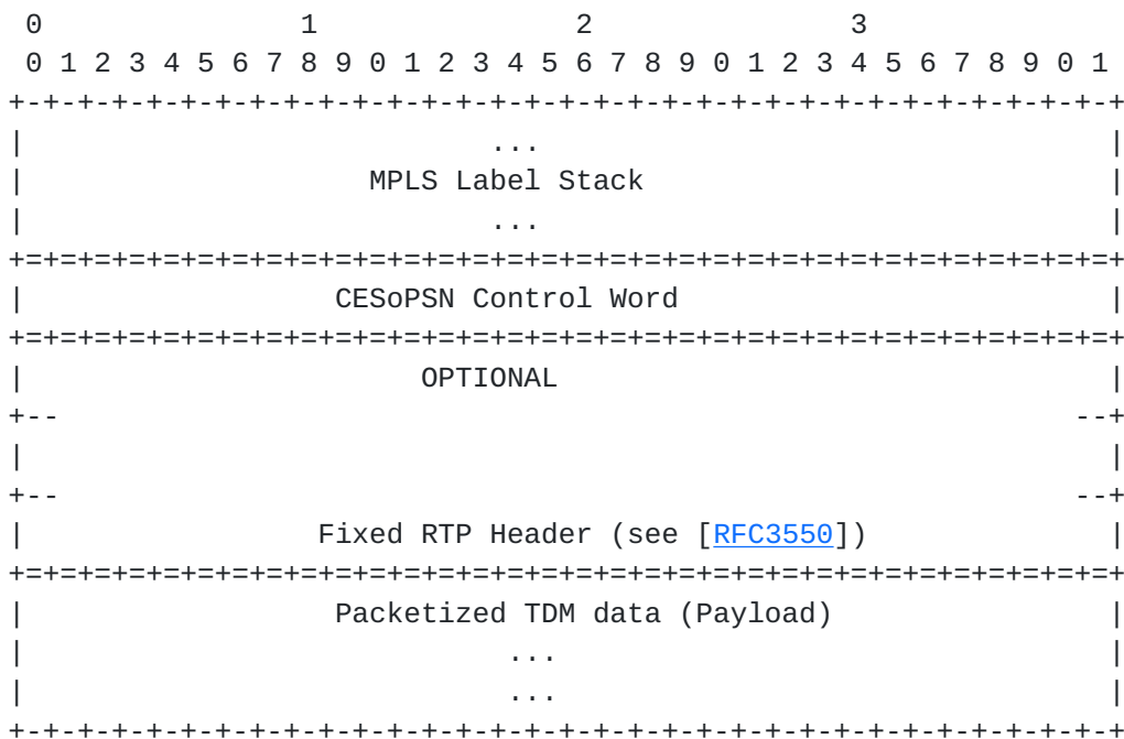
Figure 1b. CESoPSN Packet Format for an MPLS PSN
