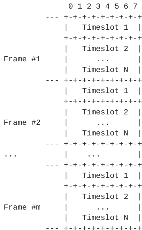
Figure 3. The CESoPSN Packet Payload Format for the Basic NxDS0 Service
