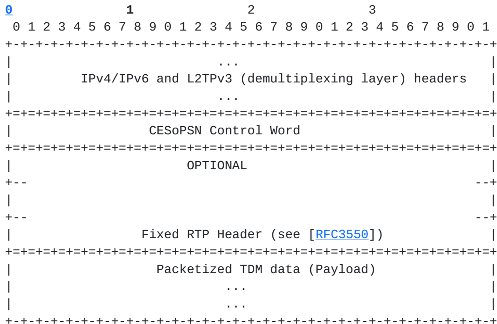
Figure 1c. CESoPSN Packet Format for an IPv4/IPv6 PSN with L2TPv3 Demultiplexing
