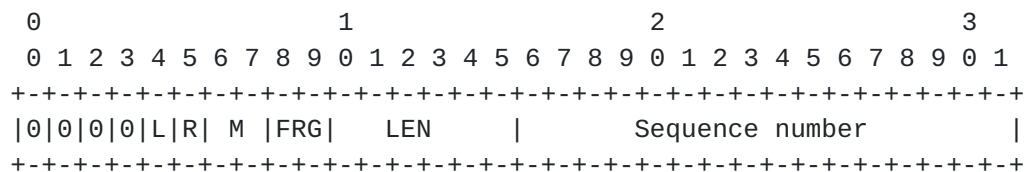
Figure 2. Structure of the CESoPSN Control Word
