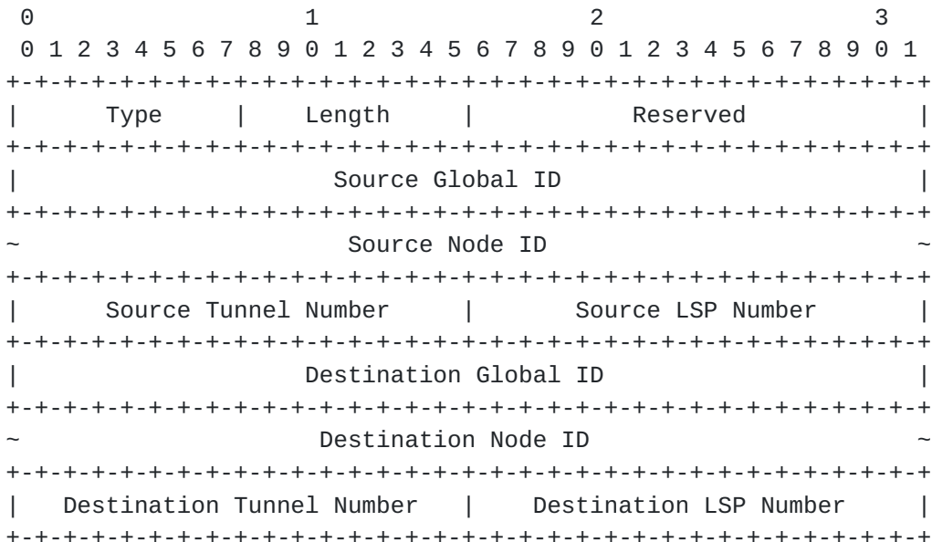
Figure 5: IPv6 PSN Tunnel sub-TLV format
