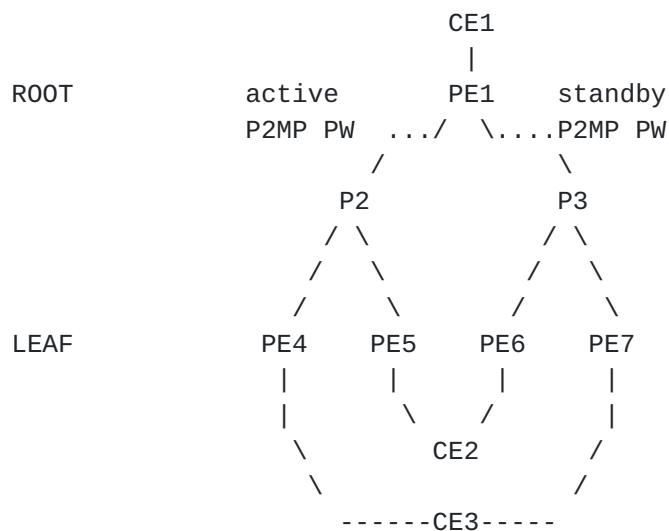
Figure 3: Example of P2MP PW redundancy for protecting Leaf PEs
