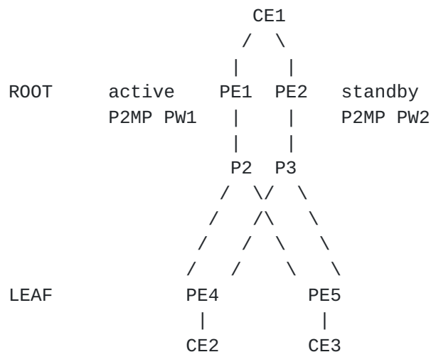
Figure 4: Example of P2MP PW redundancy for protecting Root PEs
