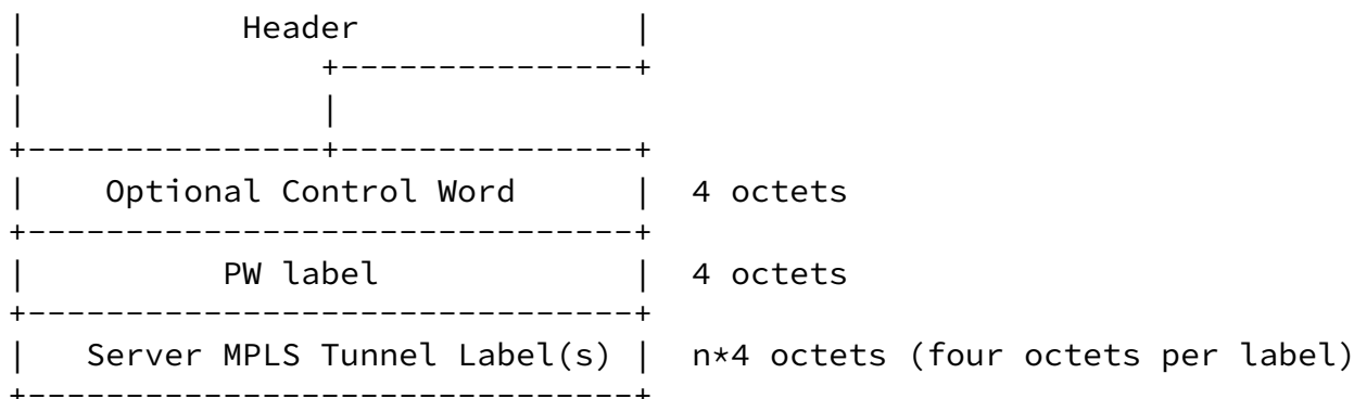
Figure 3: Packet PW Encapsulation
