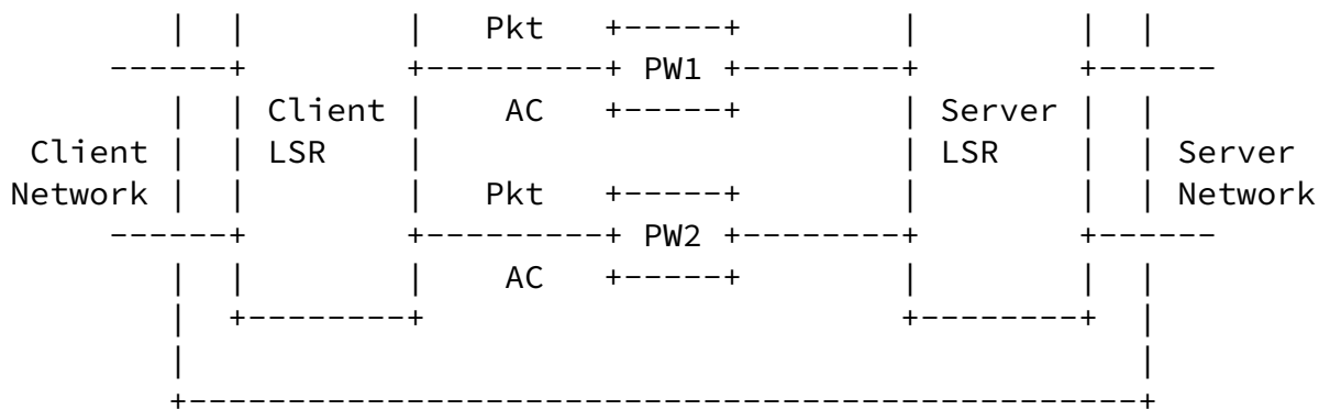
Figure 2: Packet PW Forwarding Model
