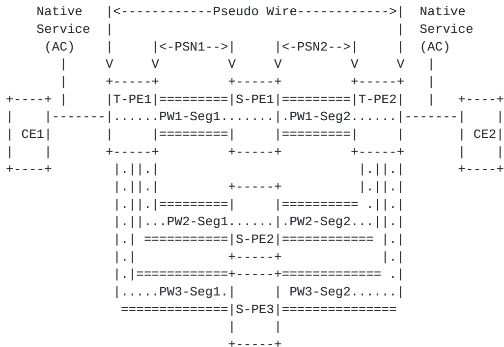
Figure 15-4 Single homed CE with multi-segment pseudo-wire redundancy
