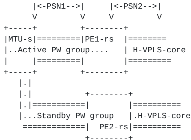
Figure 15-5 Multi-homed MTU-s in H-VPLS core
