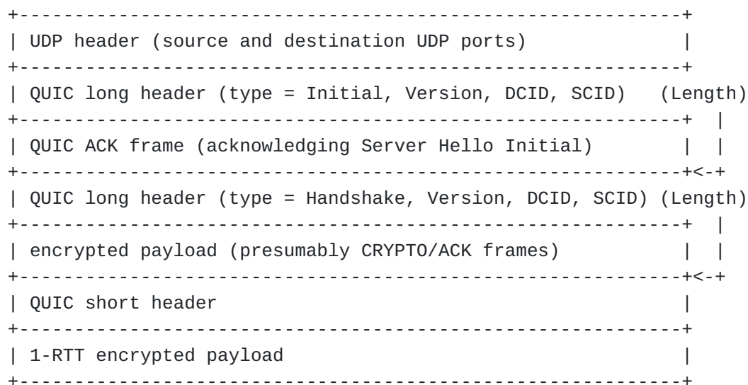
Figure 4: Typical QUIC Initial Completion datagram pattern
