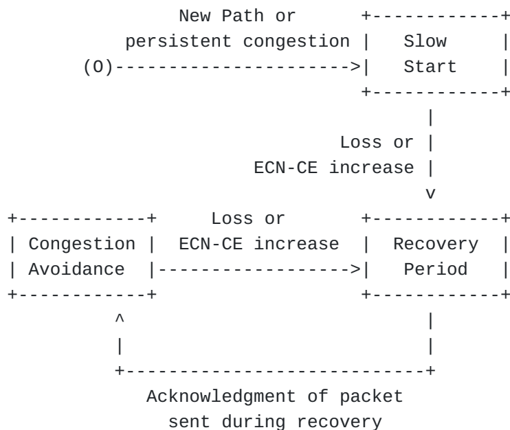
Figure 1: Congestion Control States and Transitions
