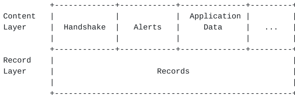
Figure 1: TLS Layers
