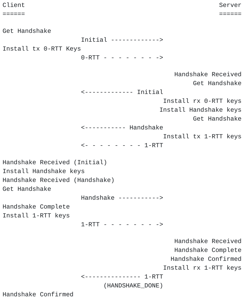
Figure 5: Interaction Summary between QUIC and TLS
