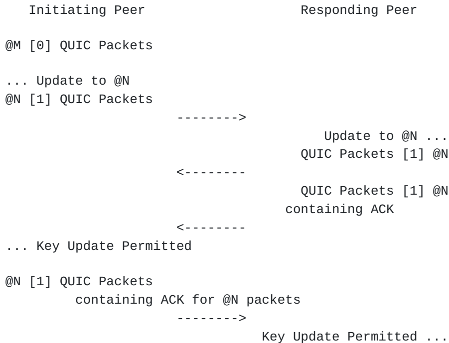
Figure 9: Key Update
