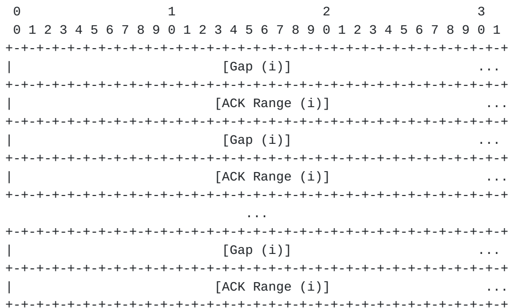
Figure 20: ACK Ranges
