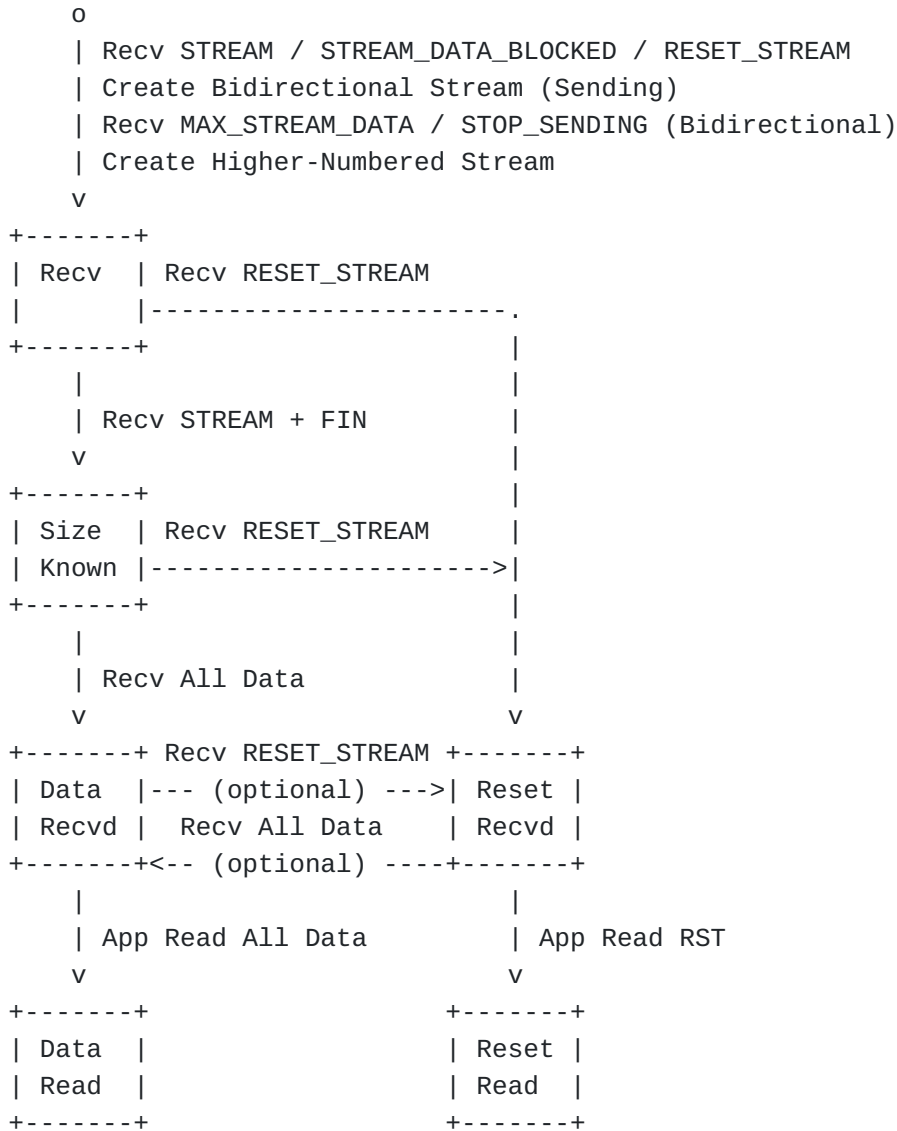
Figure 2: States for Receiving Parts of Streams
