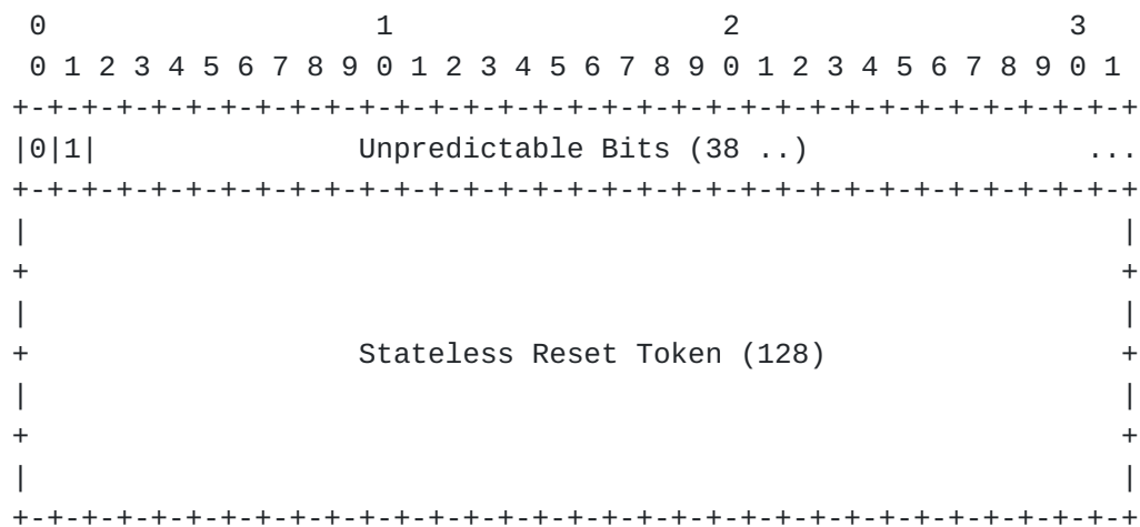
Figure 6: Stateless Reset Packet
