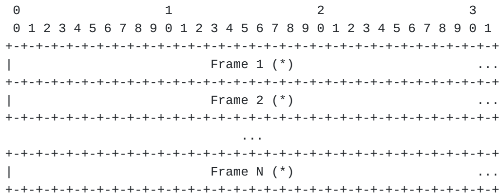
Figure 7: QUIC Payload
