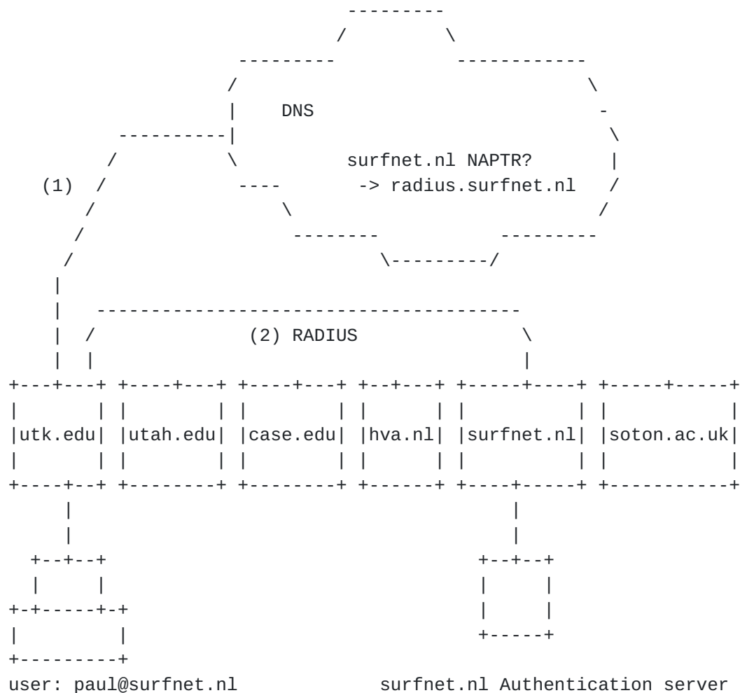
Figure 2: RADIUS hierarchy based on Top-Level Domain partitioning
