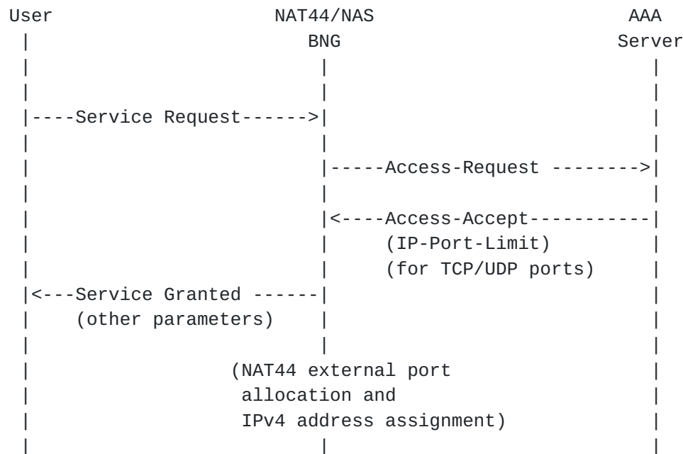
Figure 16: RADIUS Message Flow for Configuring NAT44 Port Limit
