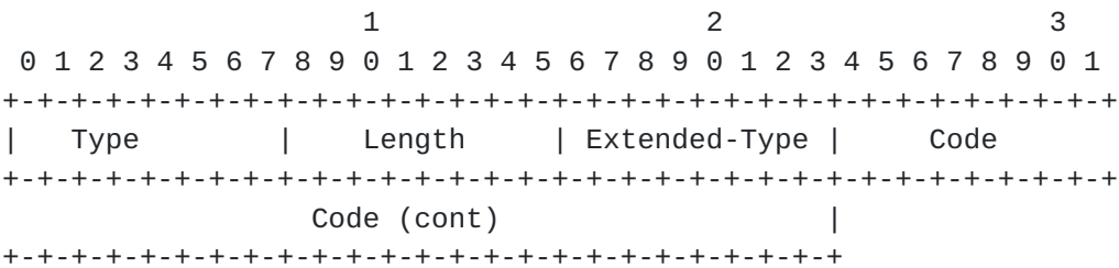
Figure 12: Frag-Status format
