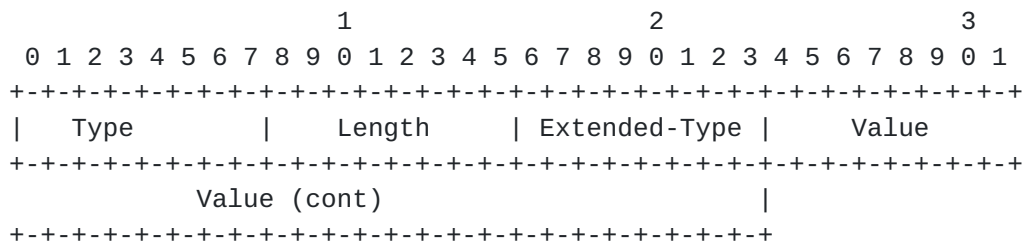
Figure 13: Proxy-State-Len format
