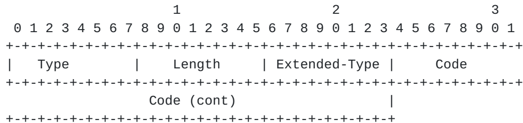
Figure 12: Frag-Status format
