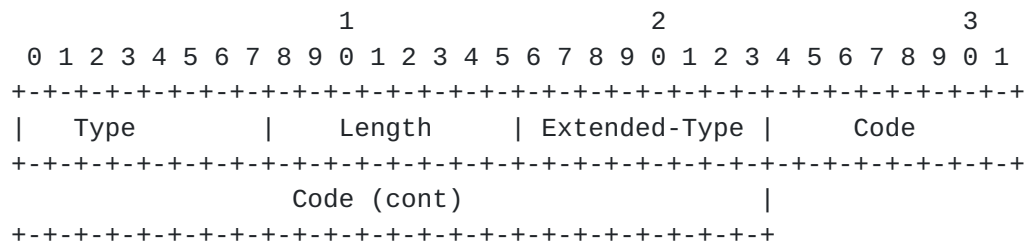
Figure 12: Frag-Status format
