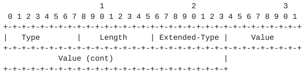
Figure 14: Proxy-State-Len format
