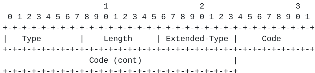
Figure 13: Frag-Status format
