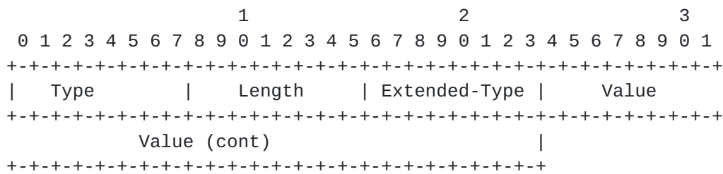
Figure 14: Proxy-State-Len format
