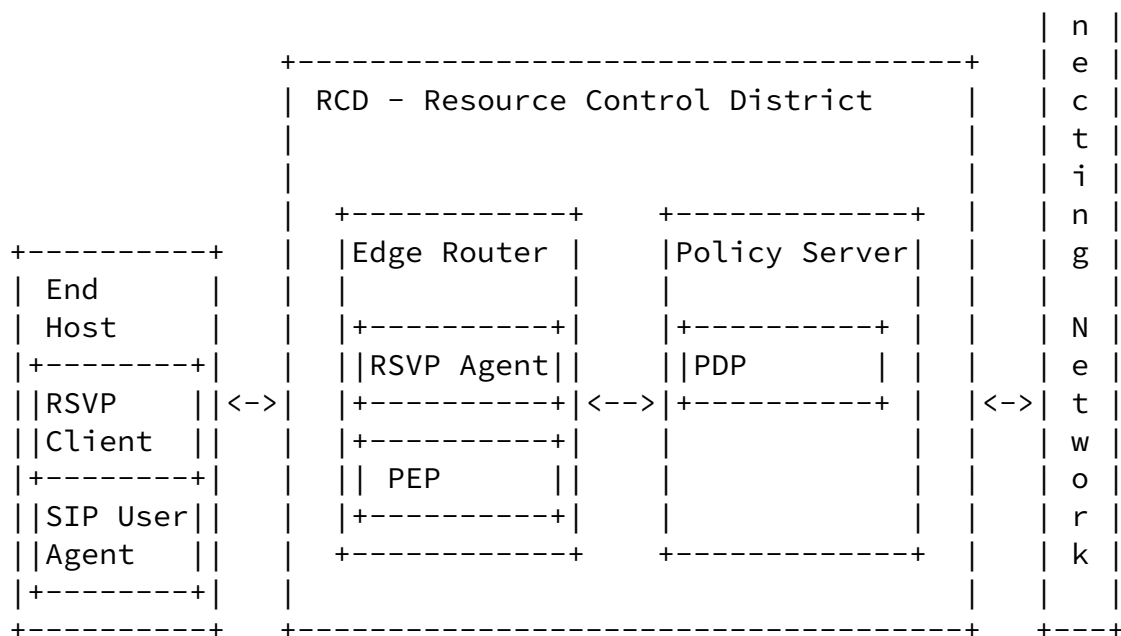
Figure 1: Generic media authorization network model
