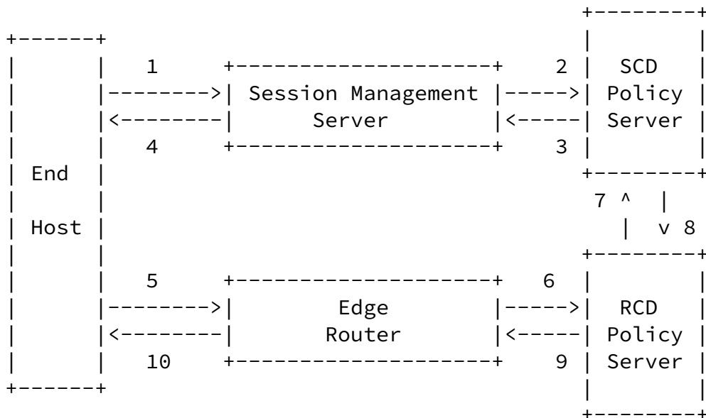
Figure 4: The Associated Model using Two Policy Servers
