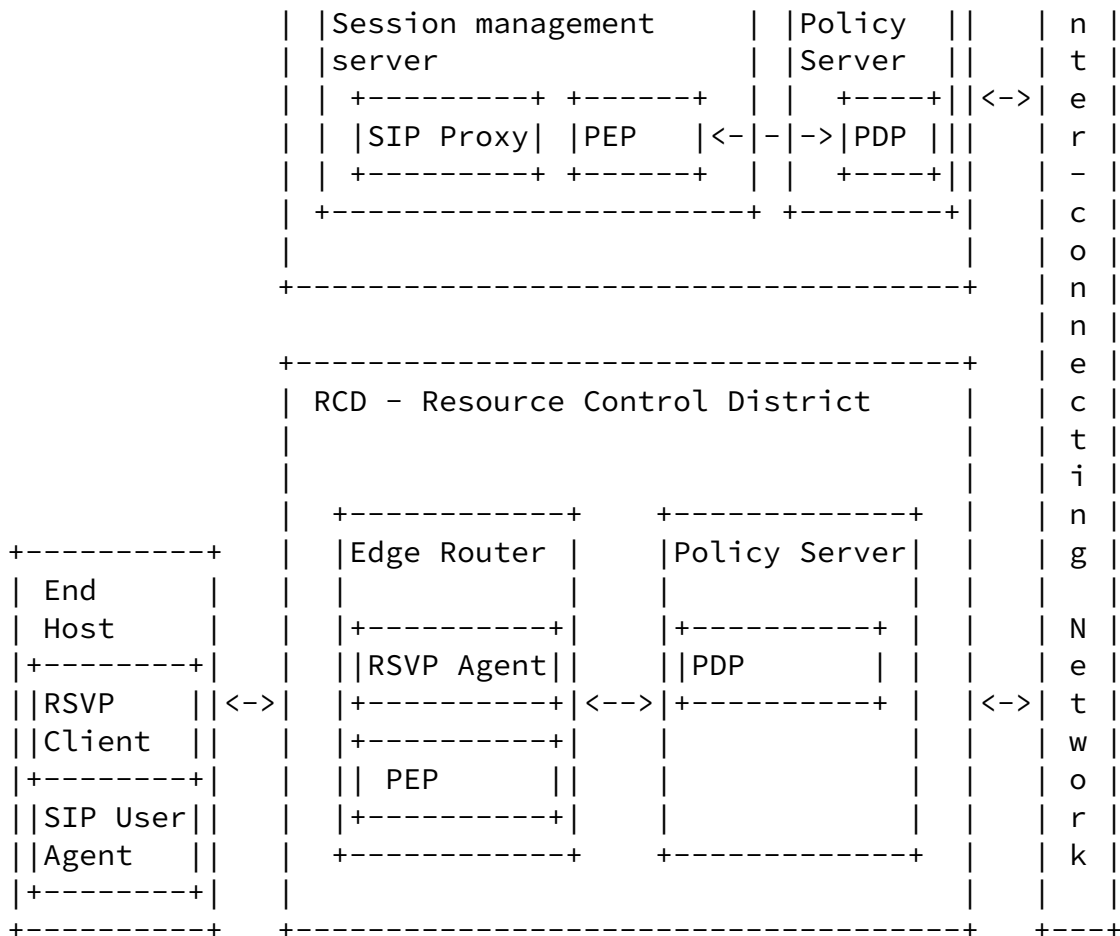
Figure 1: Generic media authorization network model
