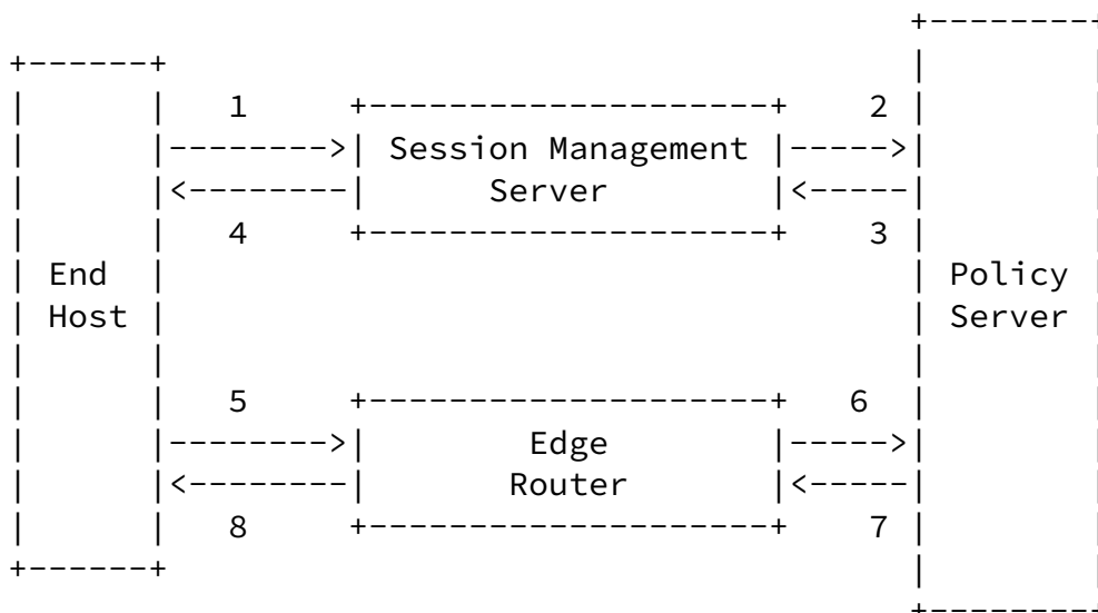
Figure 2: The Coupled Model
