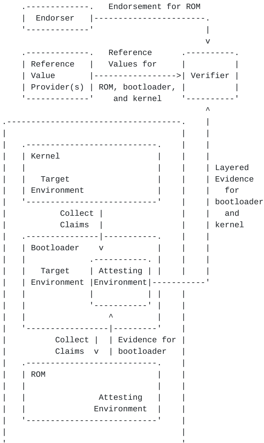
Figure 3: Layered Attester
