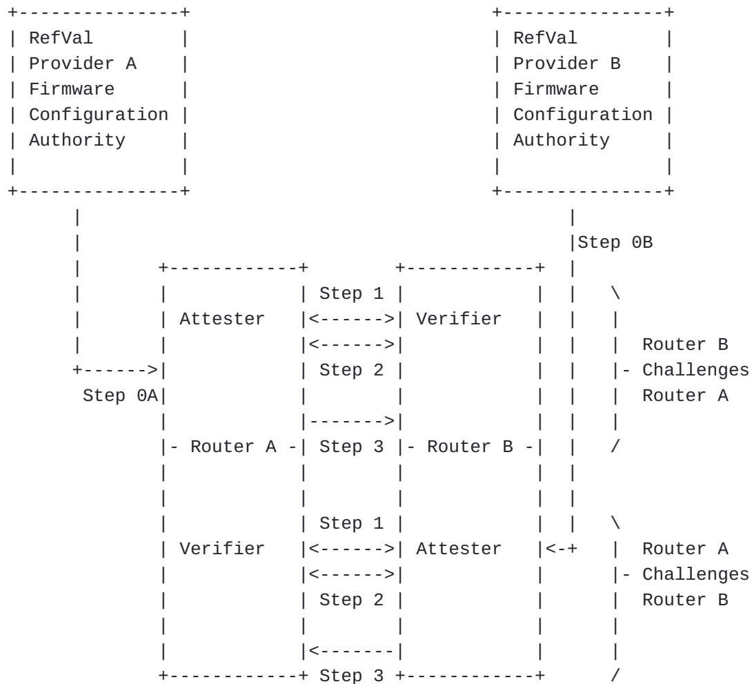
Figure 5: Peer-to-Peer Attestation Information Flow
