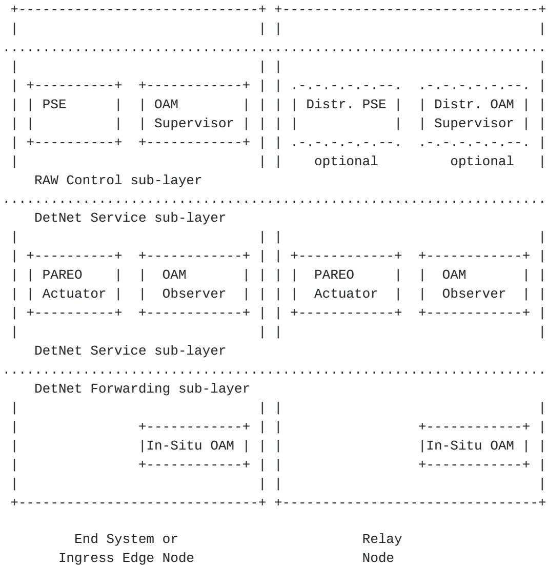
Figure 4: RAW DetNet Services
