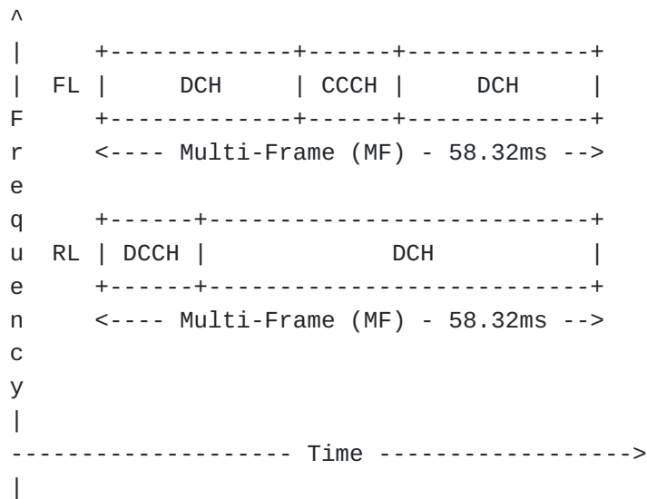
Figure 4: MF structure for LDACS
