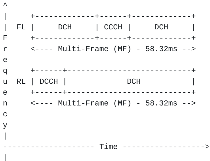
Figure 16: MF structure for LDACS
