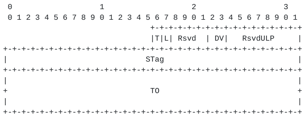
Figure 4 Tagged Buffer DDP Header
