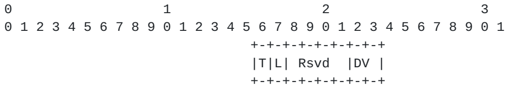
Figure 3 DDP Control Field
