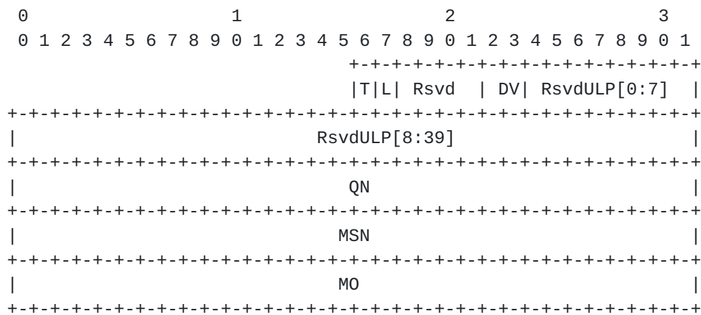
Figure 5 Untagged Buffer DDP Header
