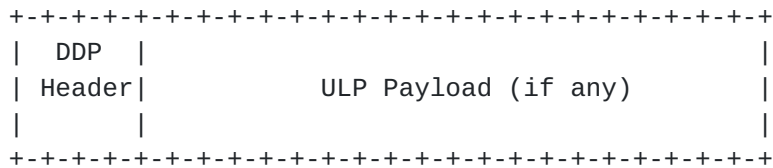
Figure 6 DDP Segment Format
