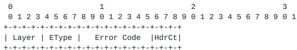
Figure 8 Terminate Control Field
