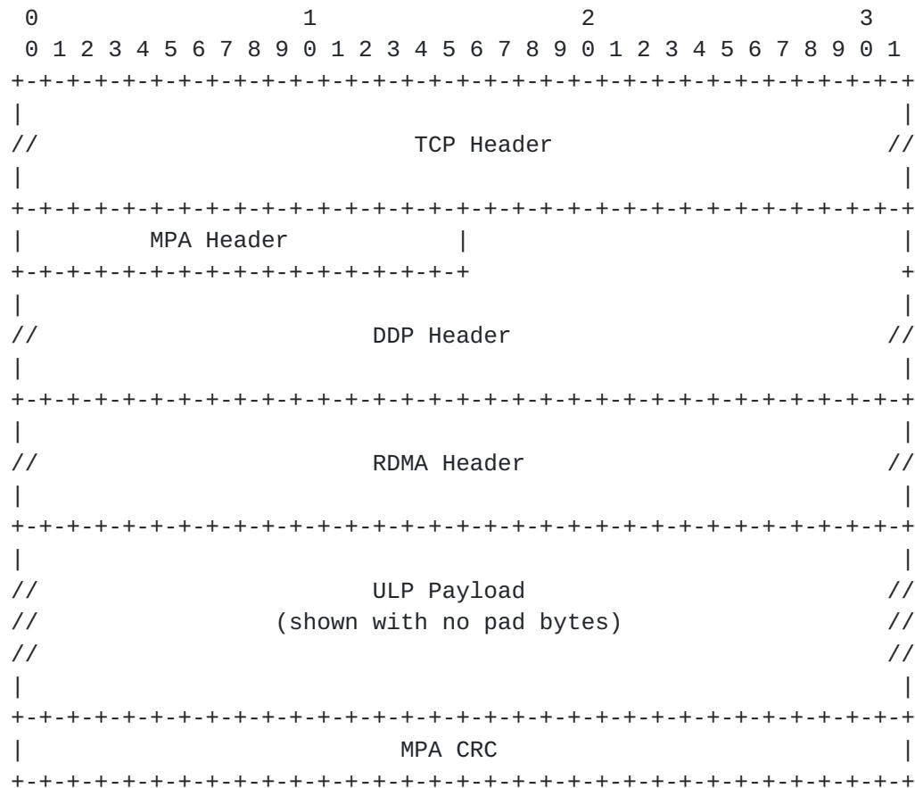
Figure 2 Example of MPA, DDP, and RDMA Header Alignment over TCP
