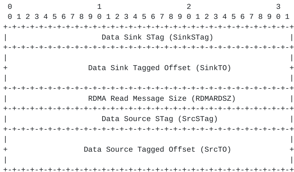
Figure 6 RDMA Read Request Header Format
