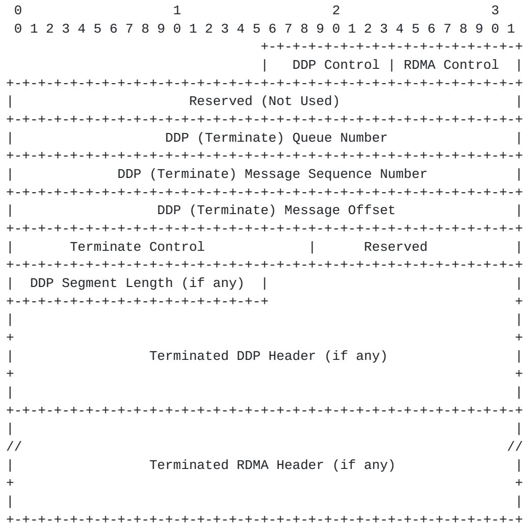
Figure 16 Terminate, DDP Segment format
