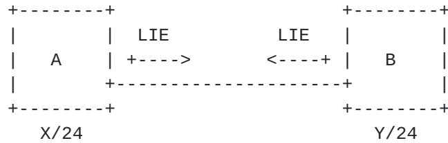
Figure 11: subnet mismatch
