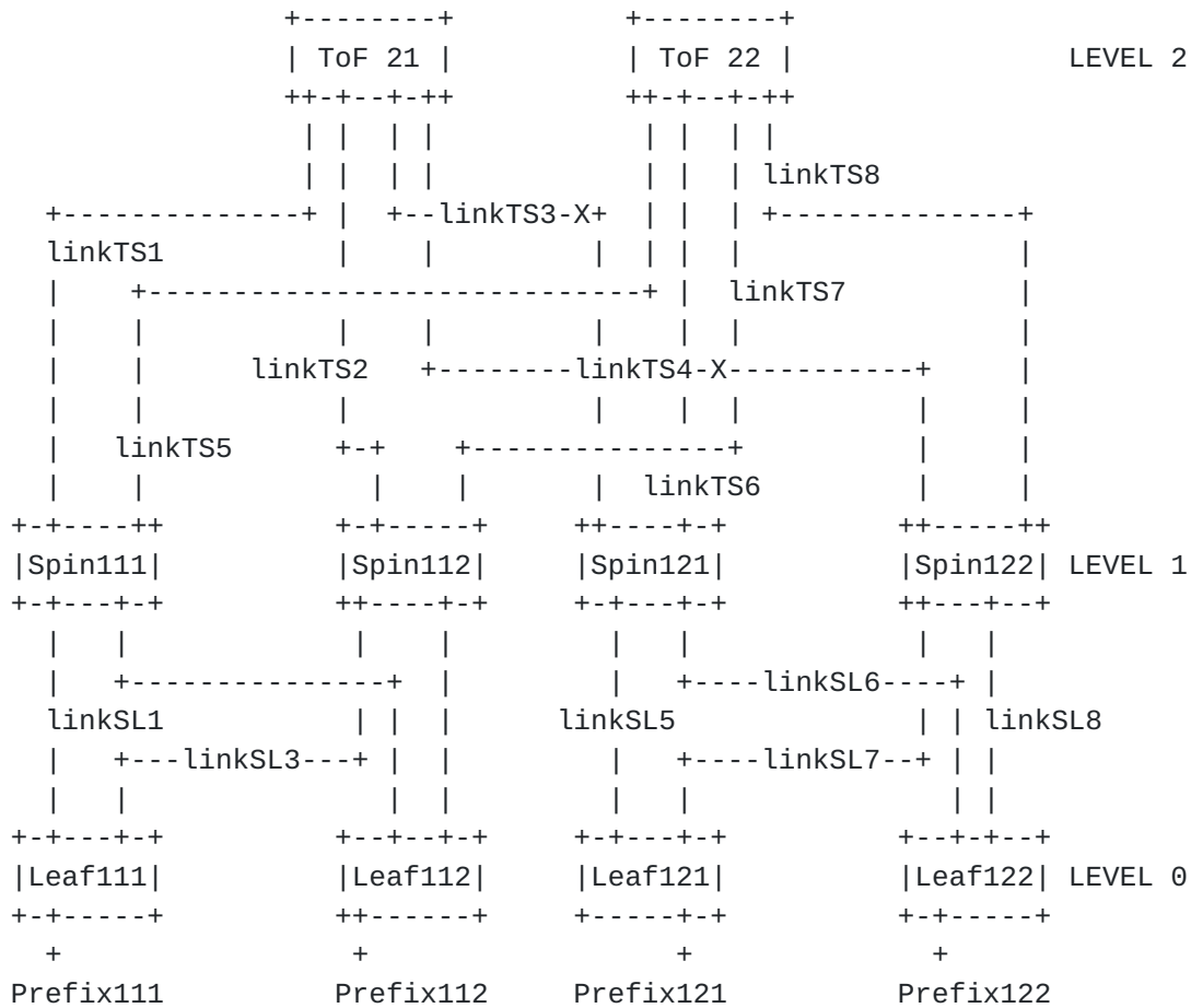
Figure 4: Black-holing upon link failure use case
