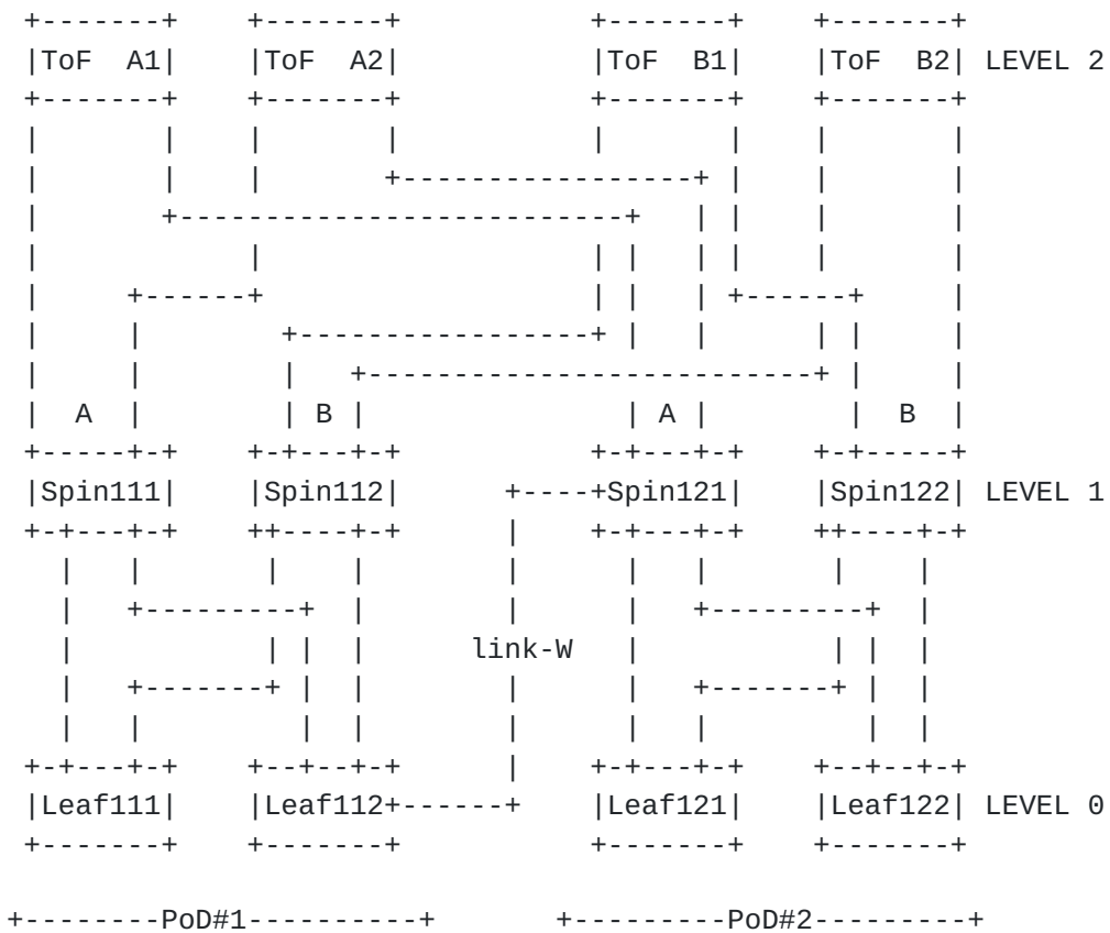
Figure 6: A multiple plane miscabling example
