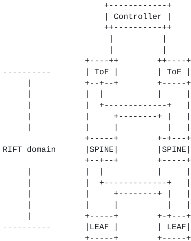
Figure 10: Fabric with a controller
