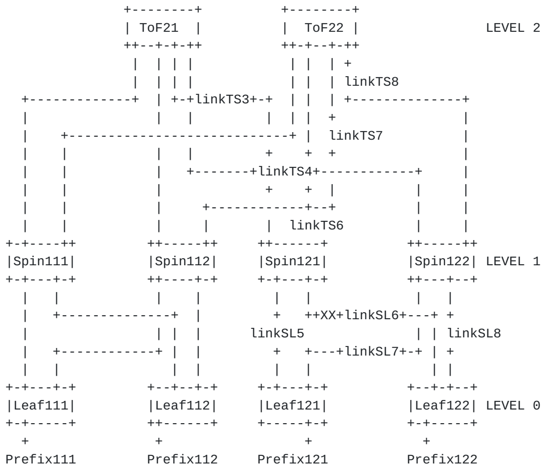
Figure 3: Suboptimal routing upon link failure use case
