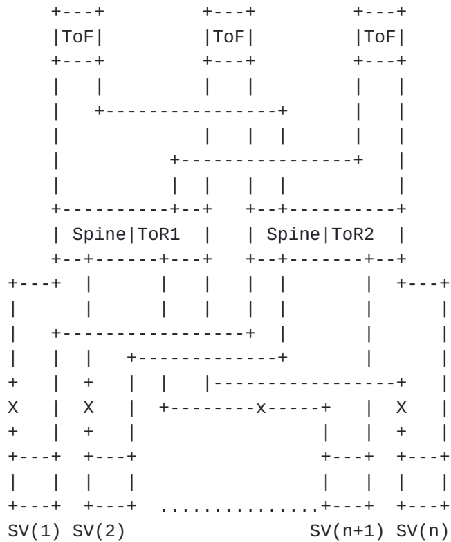
Figure 9: Dual-homing servers
