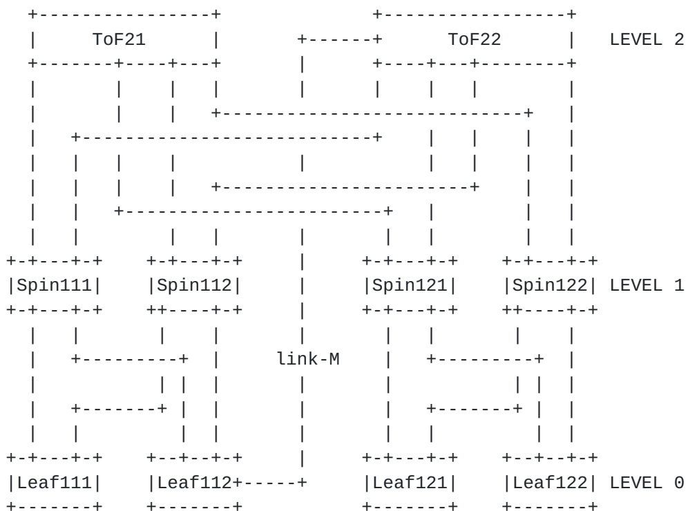
Figure 5: A single plane miscabling example
