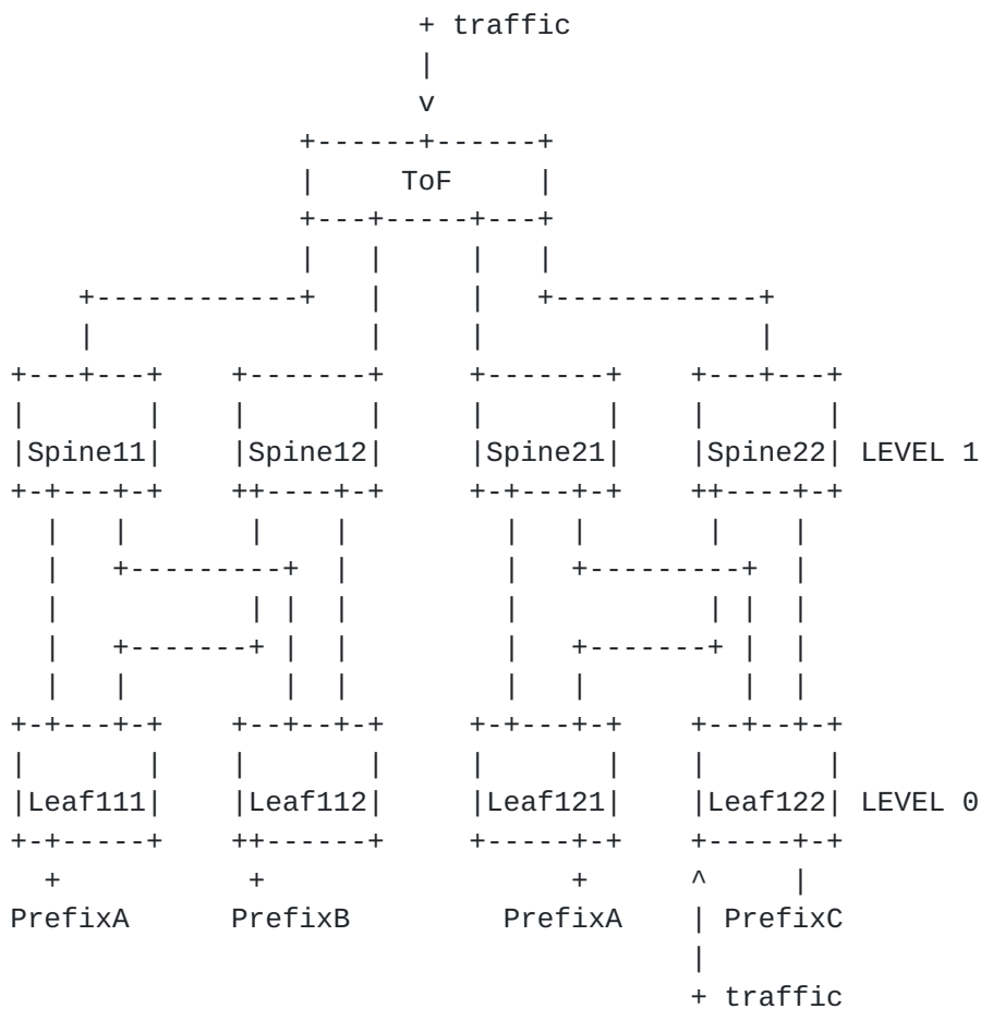
Figure 12: Anycast
