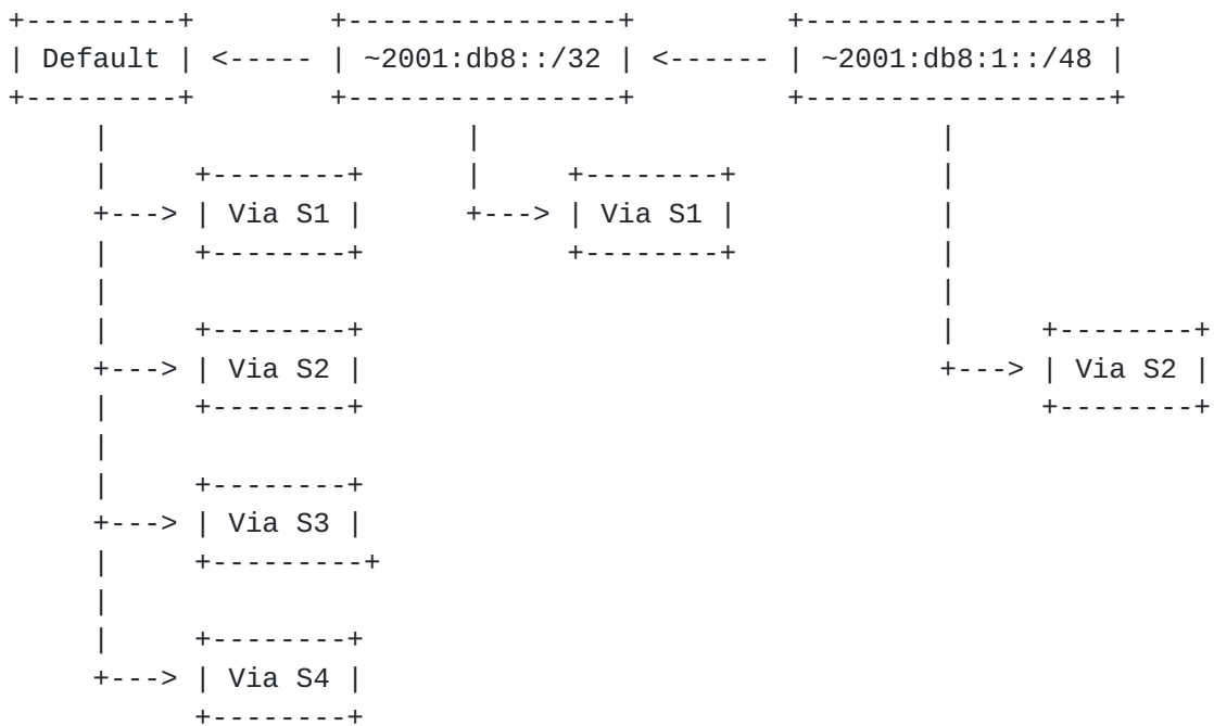
Figure 23: Abstract RIB after Negative 2001:db8:1::/48 from S2
