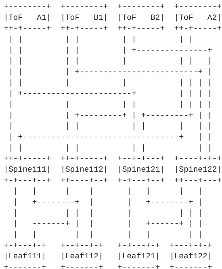
Figure 3: Topology with Multiple Planes
