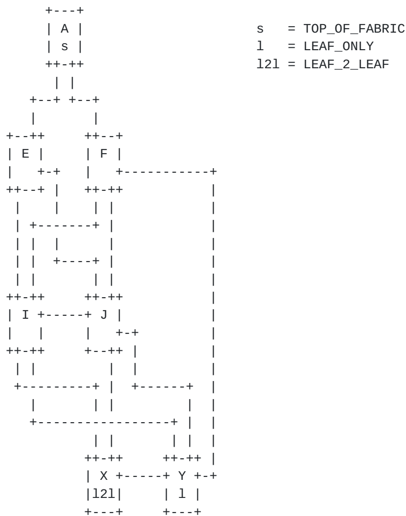
Figure 27: Generic ZTP Cabling Considerations
