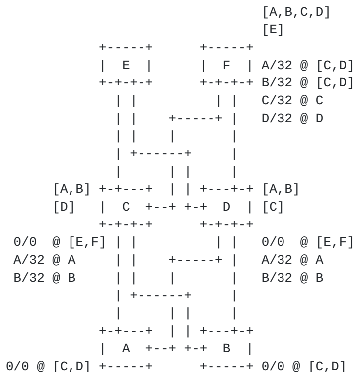
Figure 1: RIFT Information Distribution
