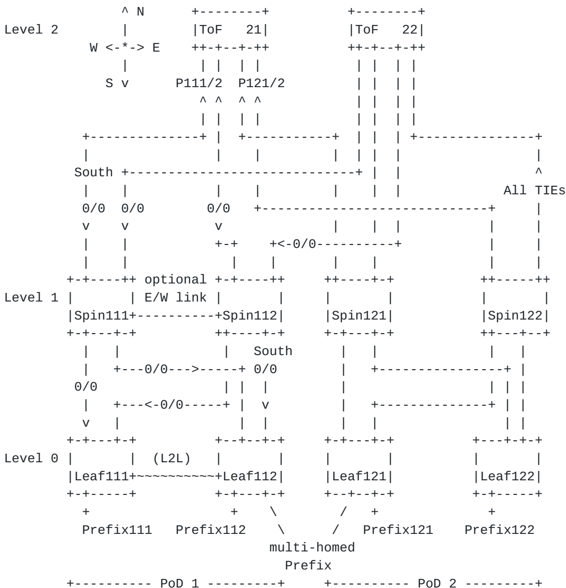
Figure 2: A Three Level Spine-and-Leaf Topology
