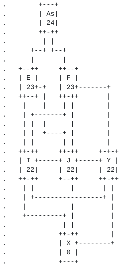
Figure 30: Generic ZTP Topology Autoconfigured
