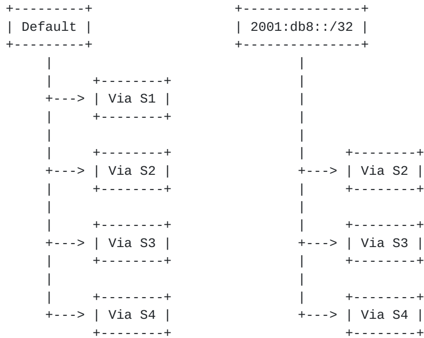
Figure 22: Abstract FIB after Negative 2001:db8::/32 from S1
