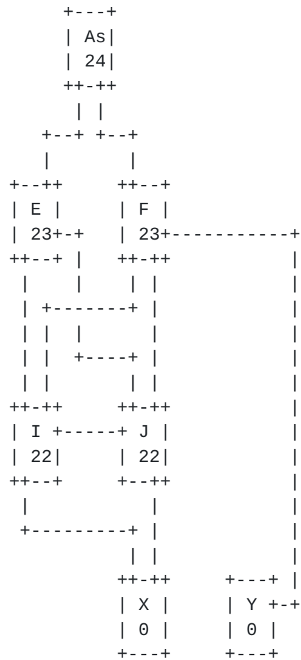
Figure 29: Generic ZTP Topology Autoconfigured
