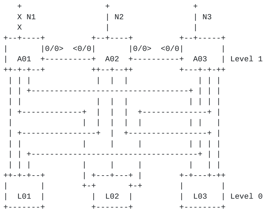
Figure 37: North Partitioned Router
