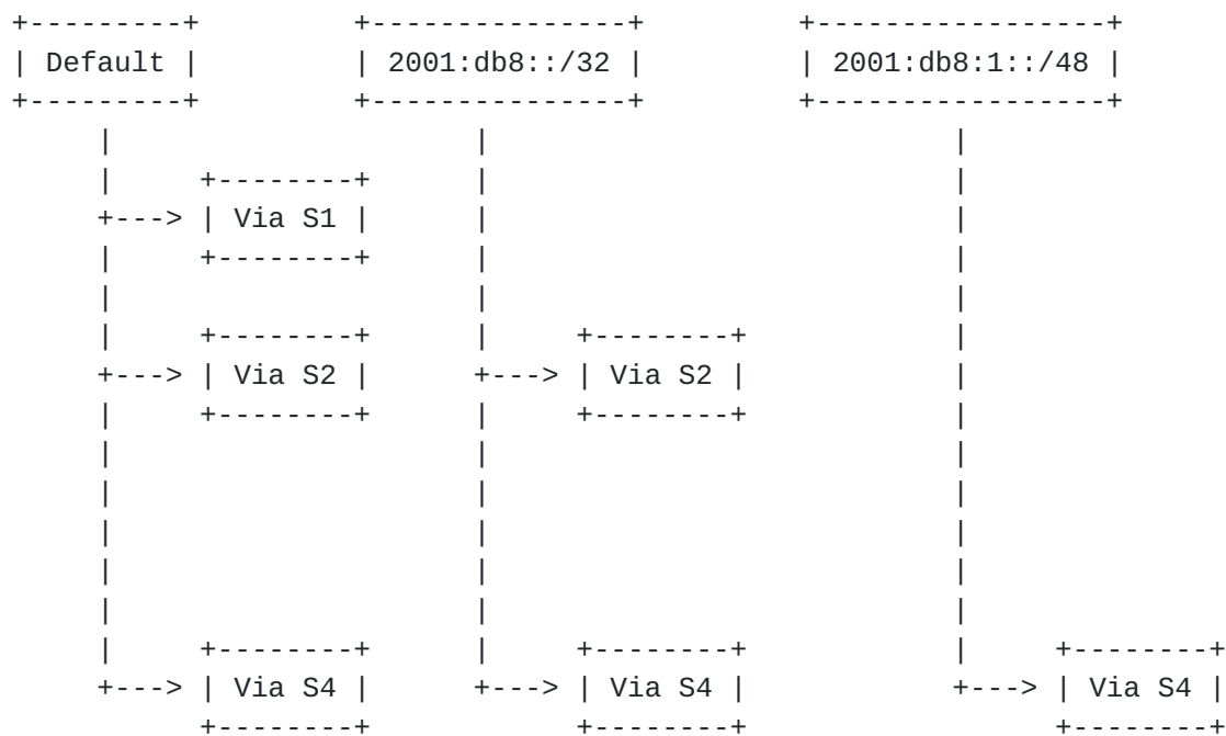
Figure 25: Abstract FIB after Loss of S3
