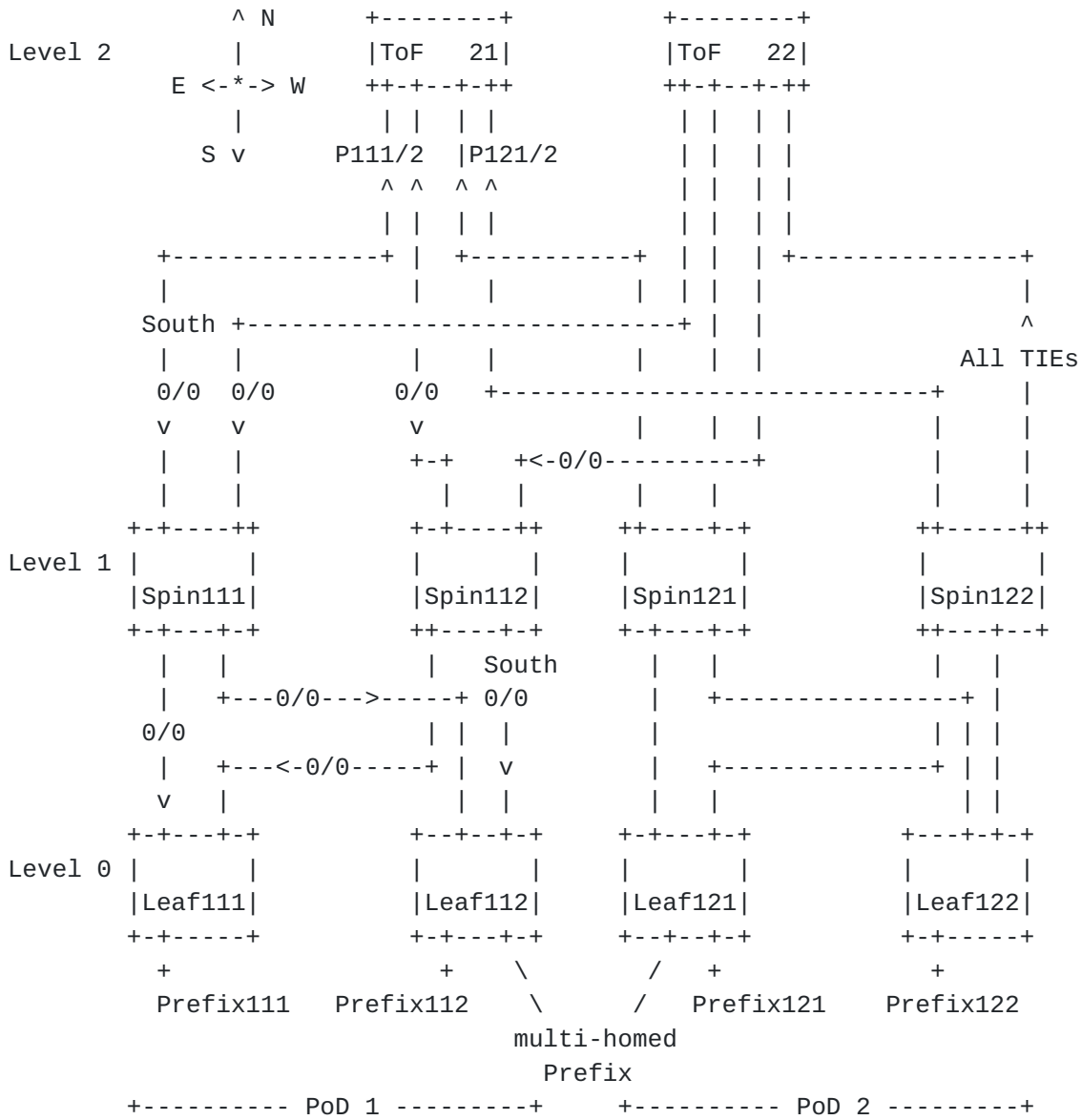
Figure 34: Normal Case Topology
