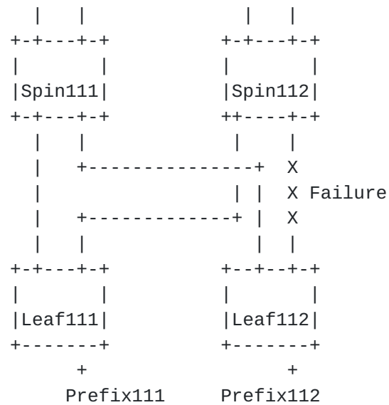
Figure 35: Single Leaf Link Failure
