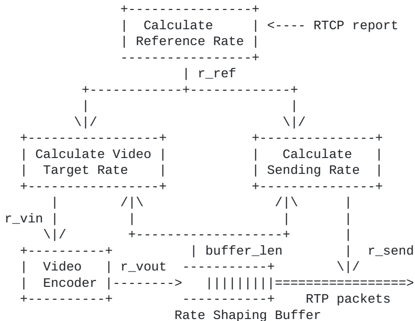
Figure 4: NADA Sender Structure
