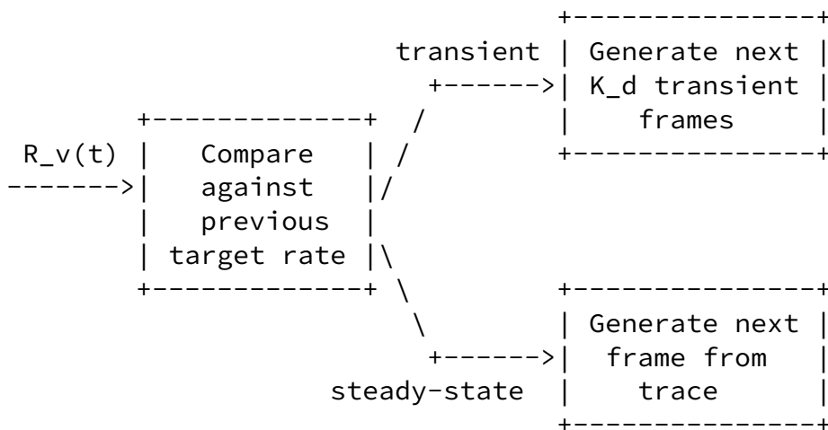
Figure 3: Hybrid approach for modeling video traffic
