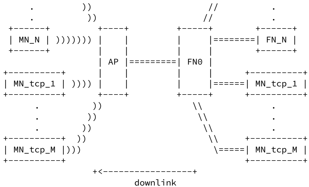
Figure 2: Network topology for Wi-Fi test cases
