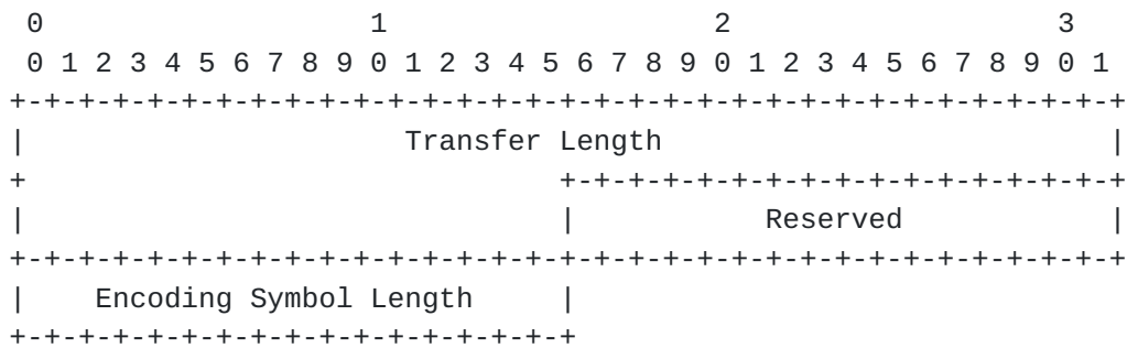
Figure 2: Encoded Common FEC OTI for Raptor FEC Scheme
