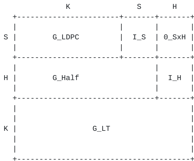
Figure 4: The matrix A
