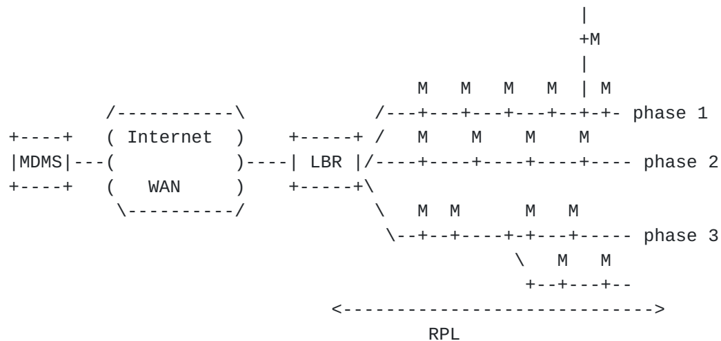
Figure 1: Typical NAN Topology
