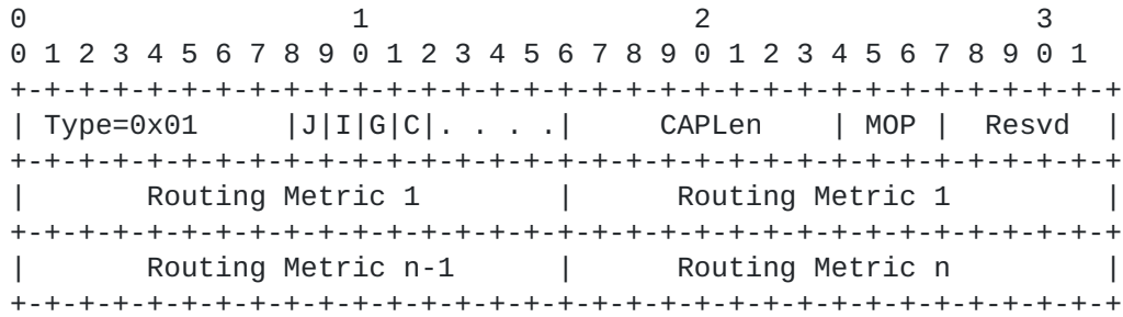
Figure 4: Projected Route Capability TLV
