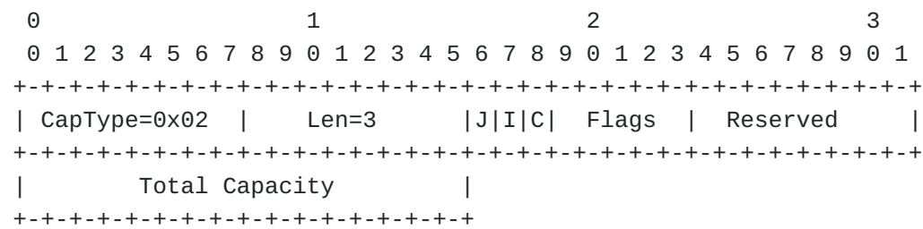
Figure 7: Routing Resource Capability TLV
