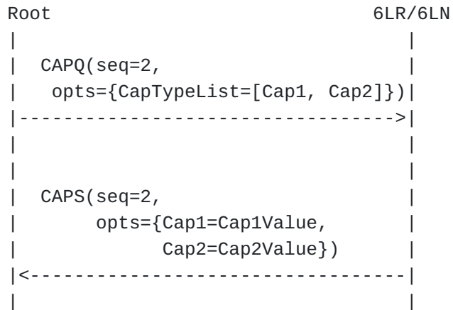
Figure 9: Query specific Cap Set
