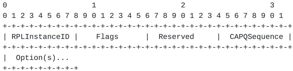
Figure 5: CAPS base object
