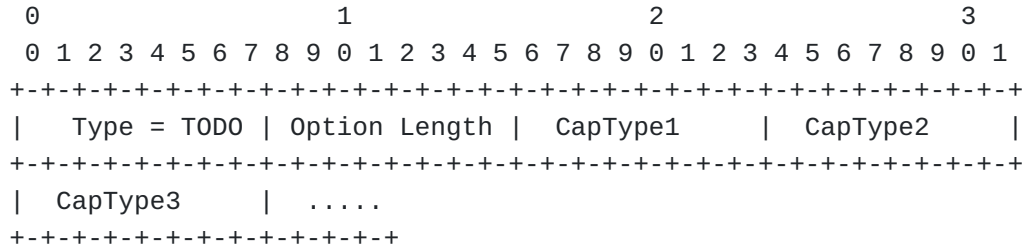
Figure 4: Capability Type List Control Option
