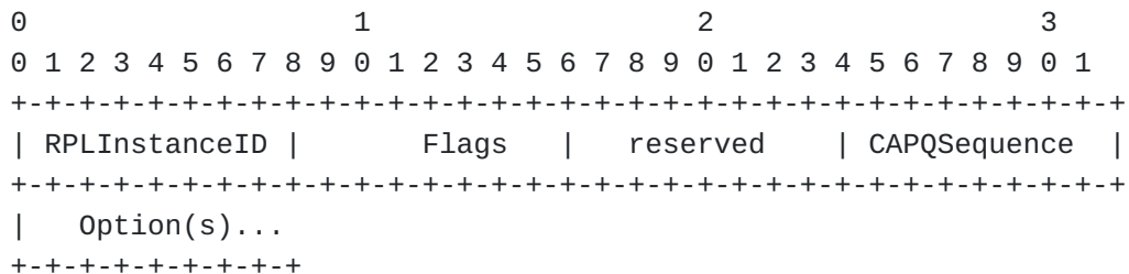
Figure 3: CAPQ base object
