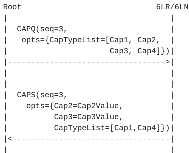
Figure 10: Partial Capability Set handshake
