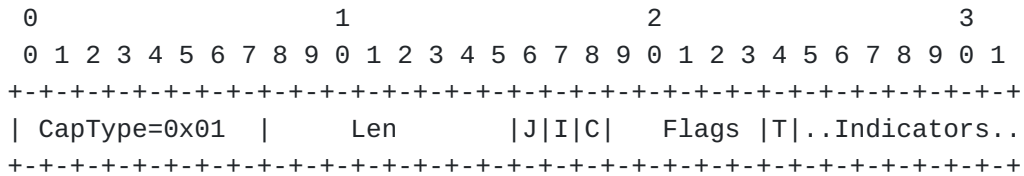
Figure 6: Capability Indicators TLV
