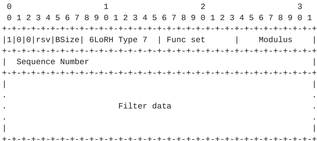
Figure 2: Routing header
