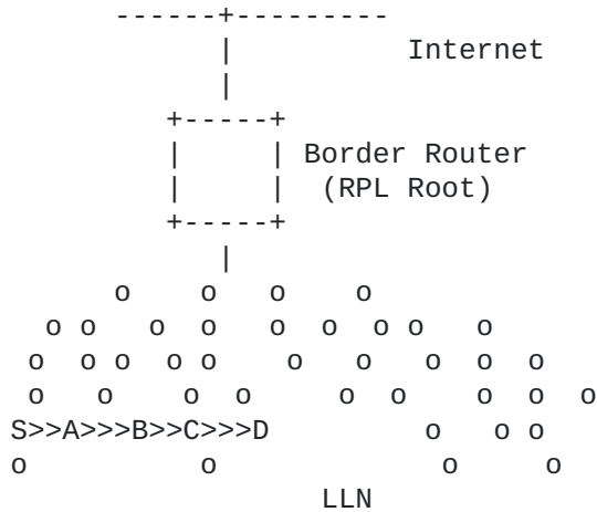
Figure 10: Projected Transversal Route
