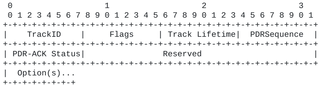
Figure 2: New PDR-ACK Control Message Format
