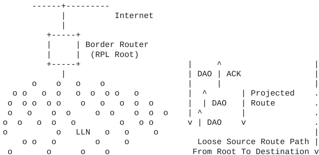
Figure 7: Projecting a route
