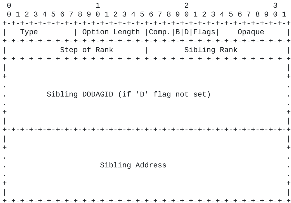
Figure 5: Sibling Information Option Format
