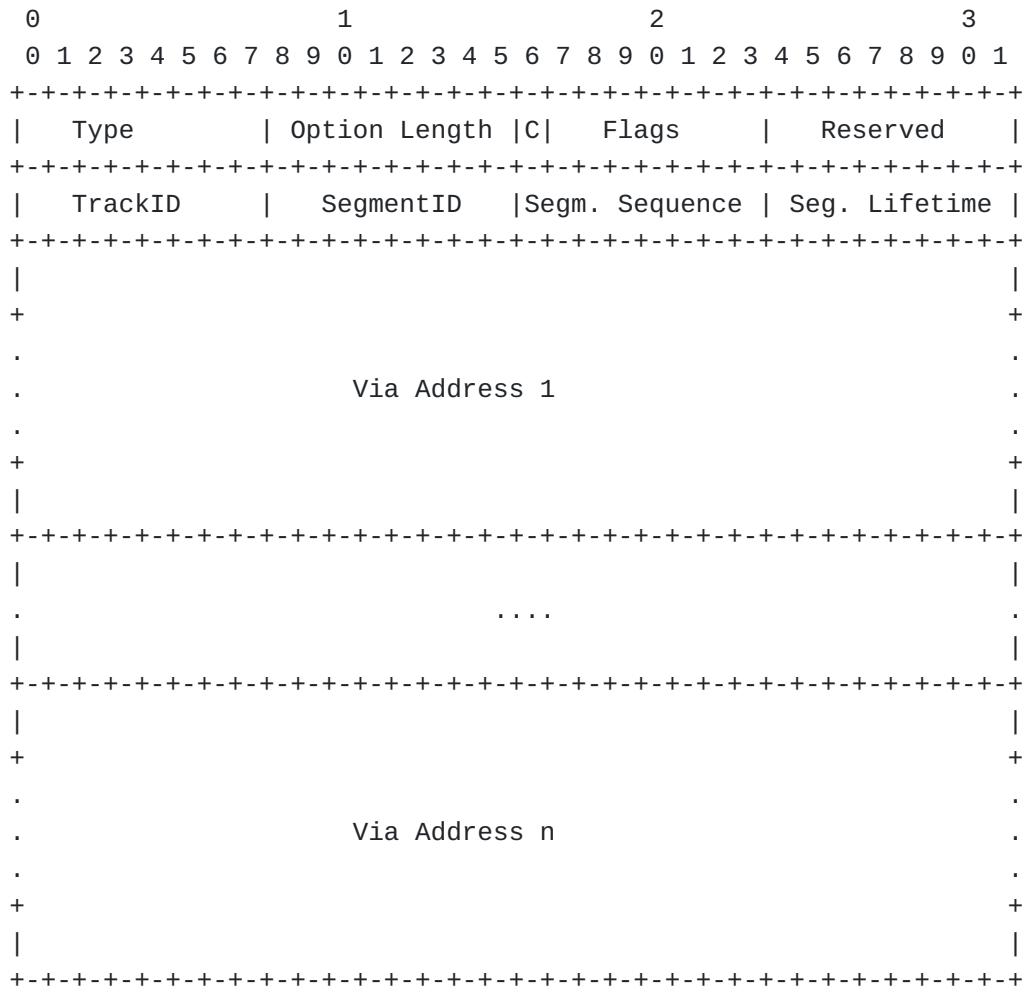
Figure 4: Via Information option format (uncompressed form)
