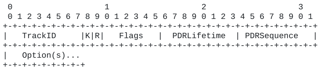
Figure 1: New P-DAO Request Format
