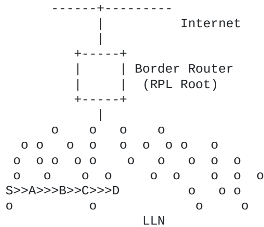
Figure 14: Projected Transversal Route
