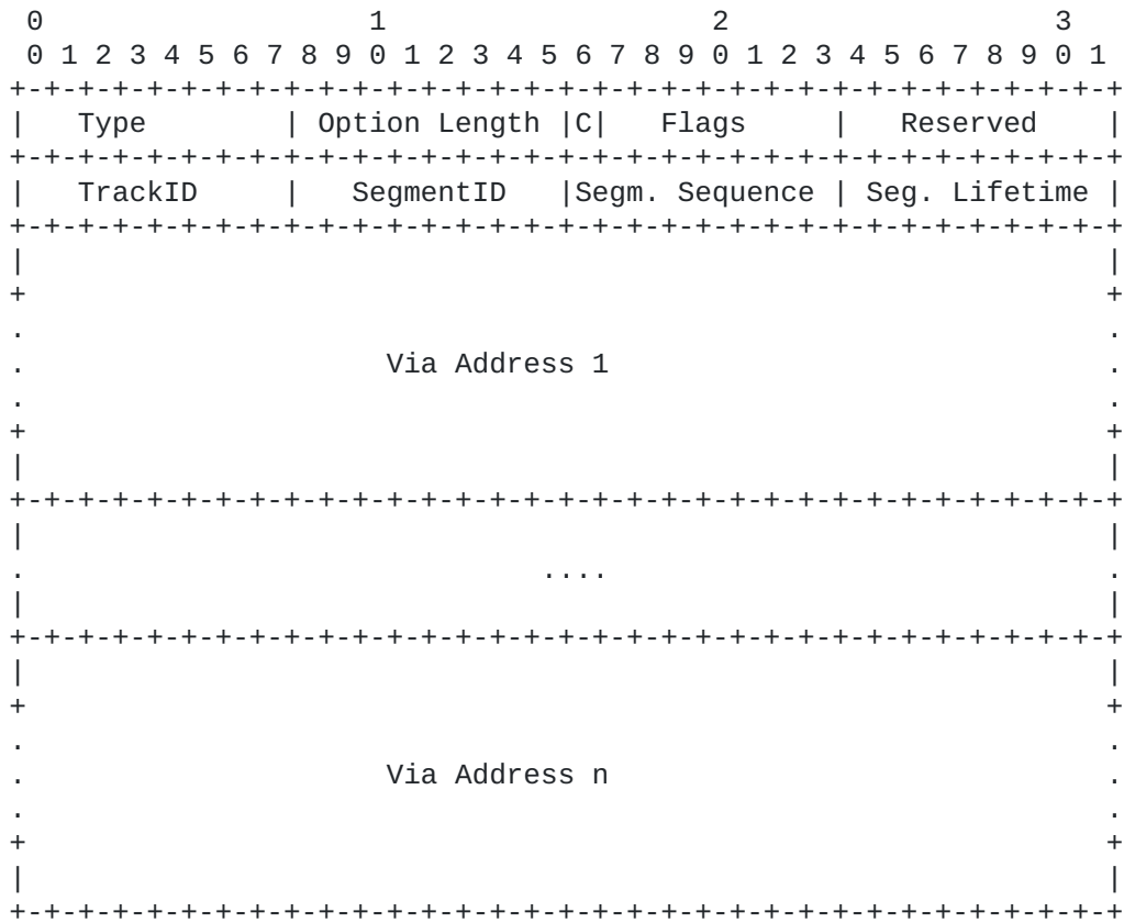
Figure 4: Via Information option format (uncompressed form)
