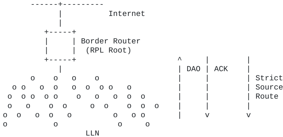
Figure 8: RPL non-storing mode of operation
