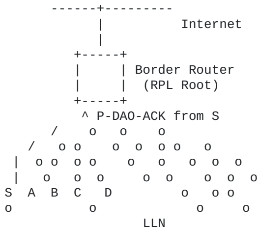
Figure 13: P-DAO-ACK to Root
