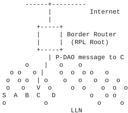
Figure 12: P-DAO from Root
