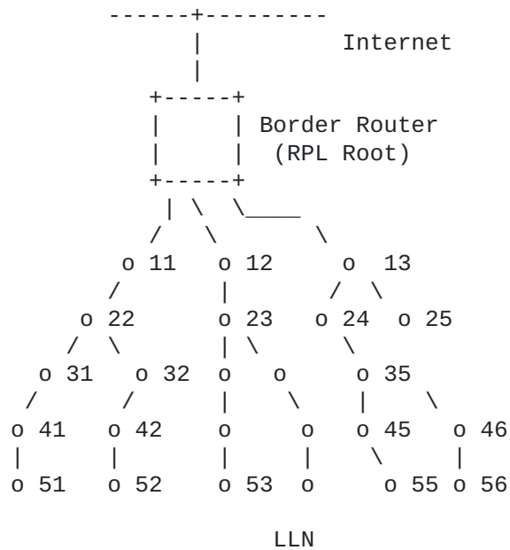
Figure 11: Example DODAG forming a logical tree topology
