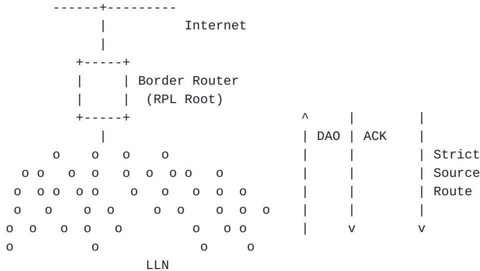
Figure 8: RPL non-storing mode of operation
