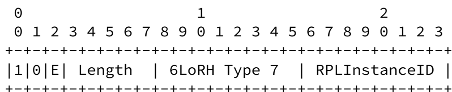
Figure 3: P-RPI-6LoRH Format
