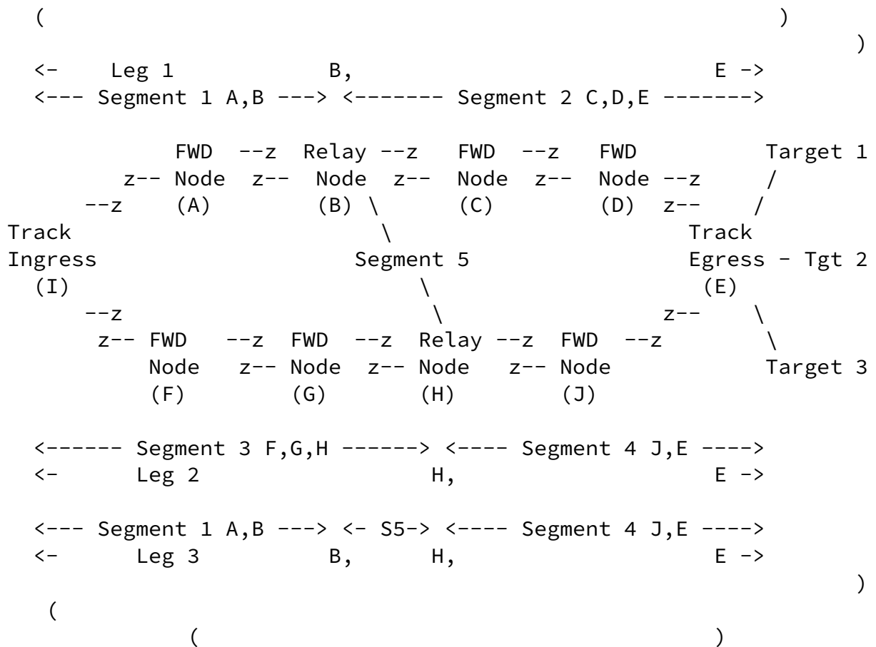
Figure 5: Segments and Tracks
