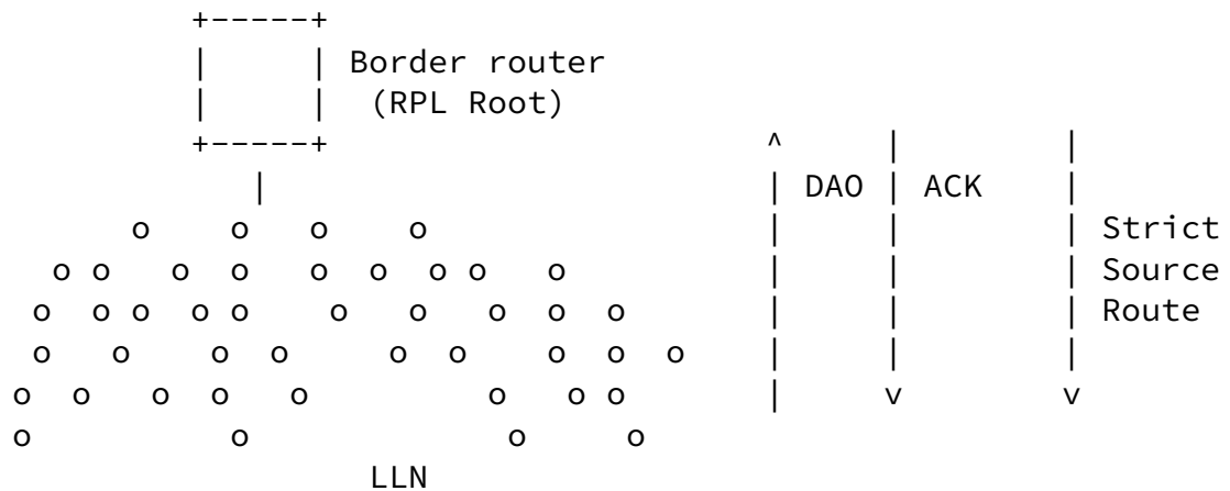
Figure 1: RPL Non-Storing Mode of operation
