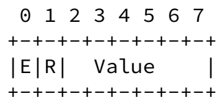
Figure 11: PDR-ACK status Format
