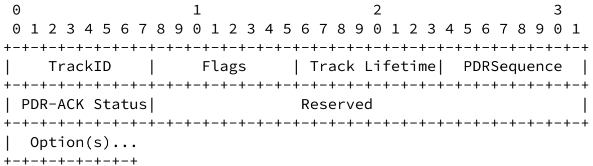
Figure 10: New PDR-ACK Control Message Format
