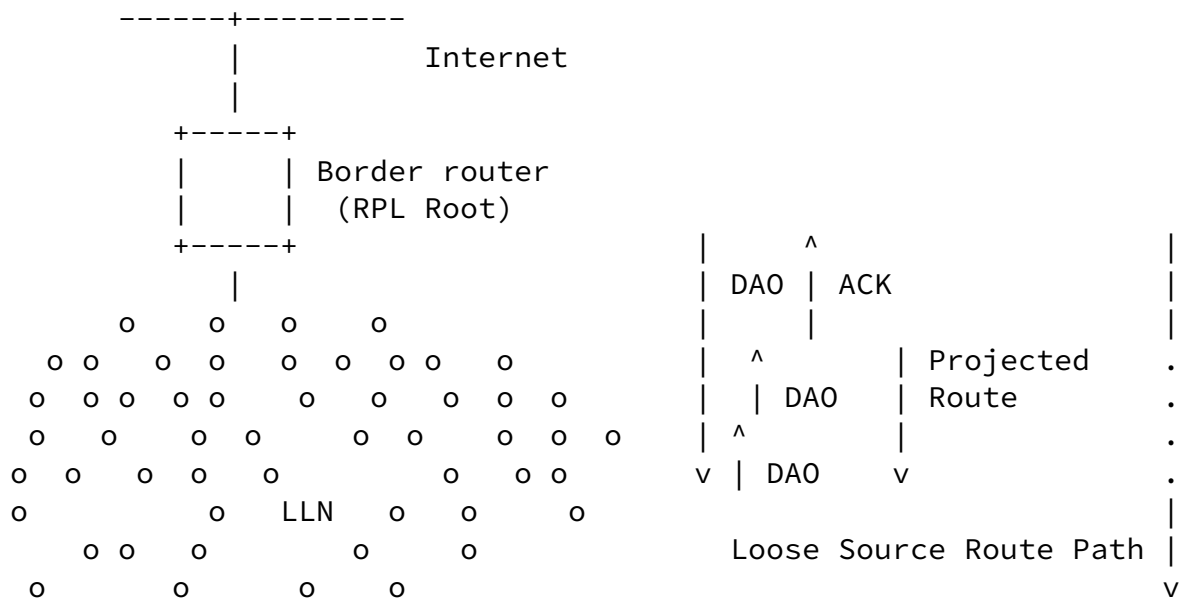
Figure 14: Projecting a route
