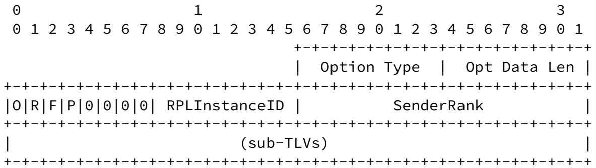
Figure 7: Extended RPL Option Format
