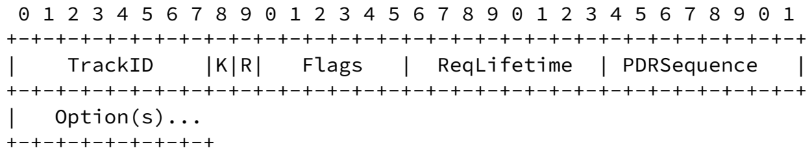
Figure 9: New P-DAO Request Format
