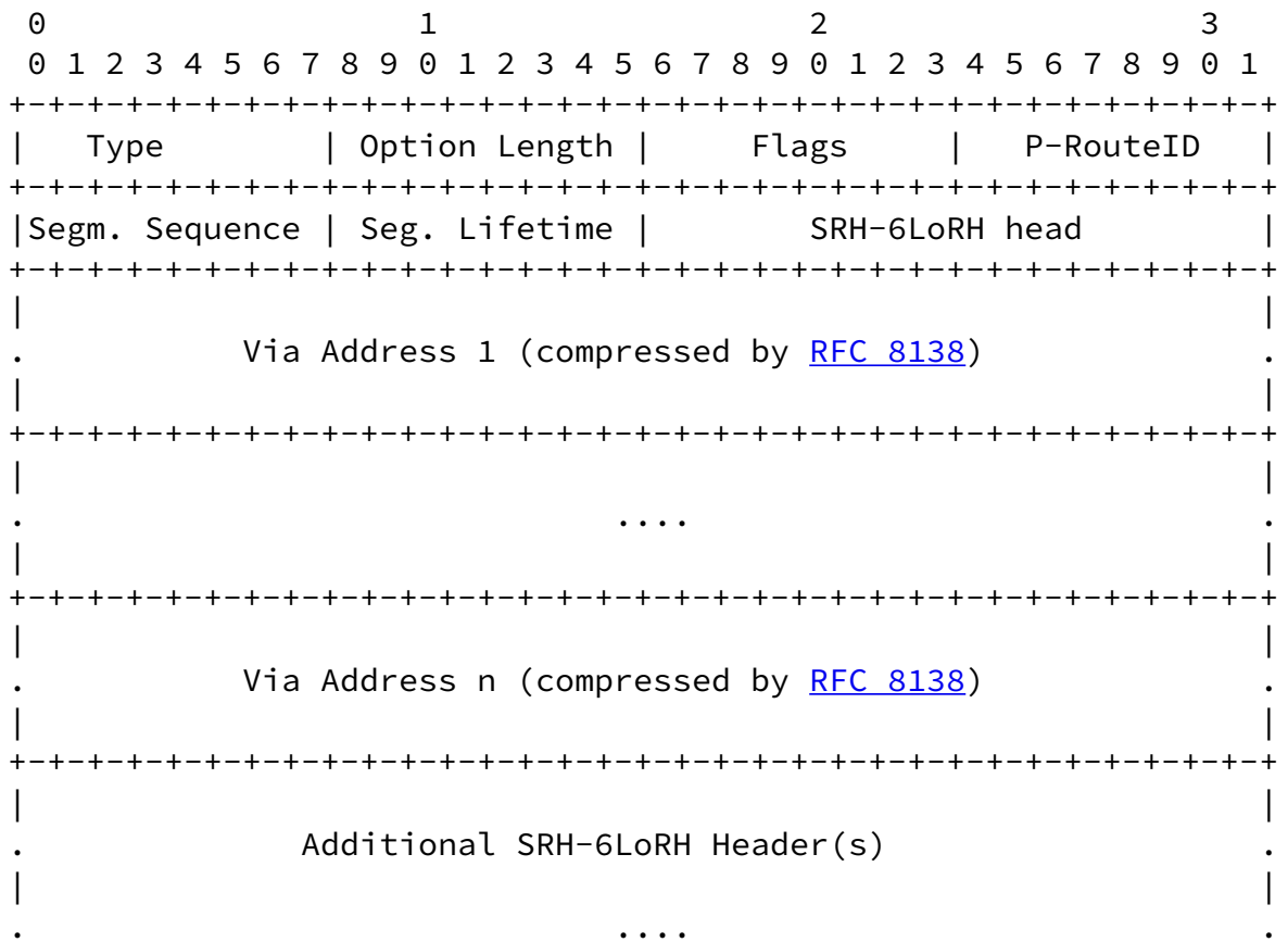
Figure 12: VIO format (uncompressed form)
