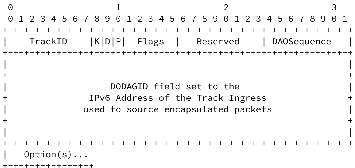
Figure 6: Projected DAO Base Object
